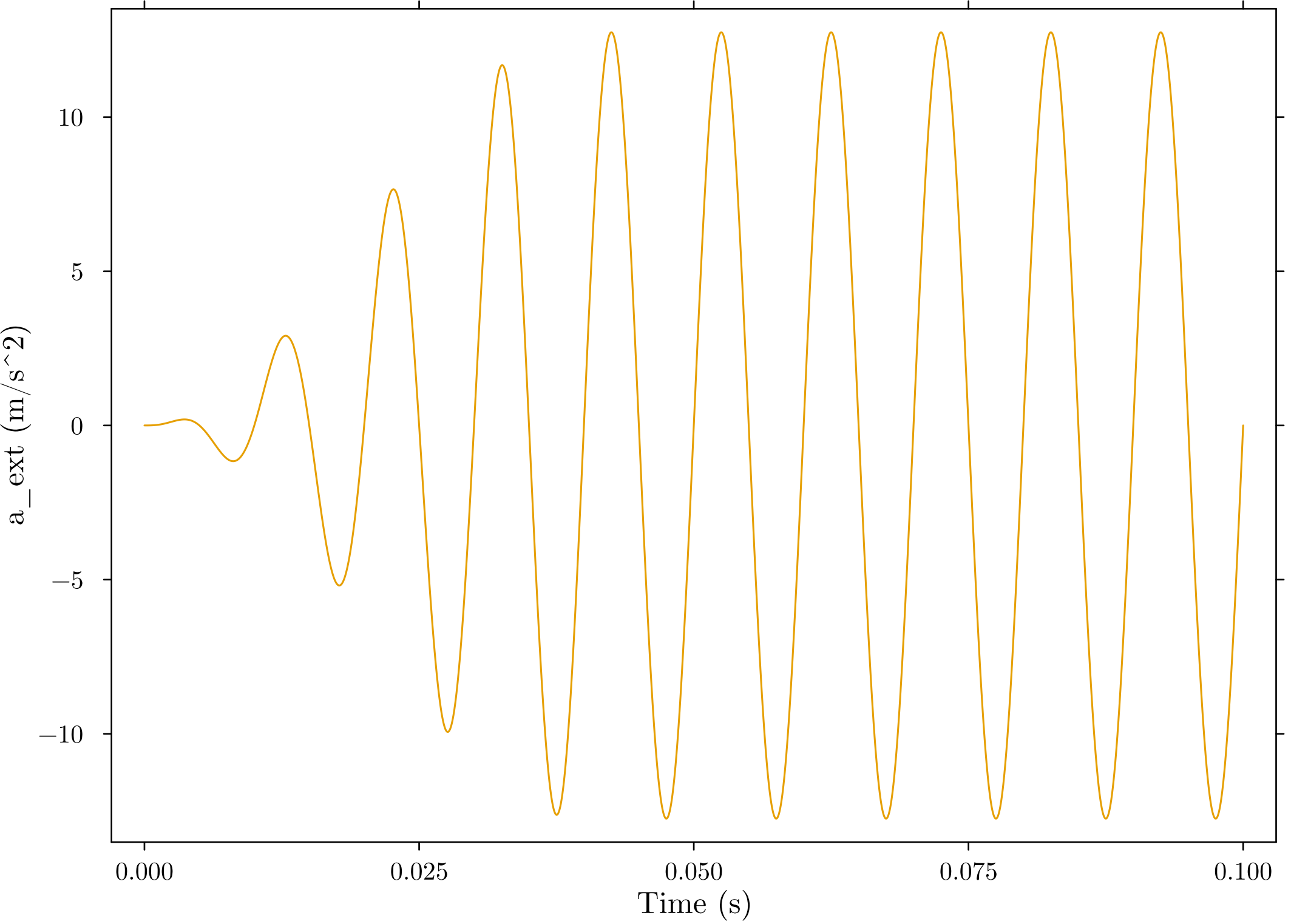
Applied Base Acceleration
