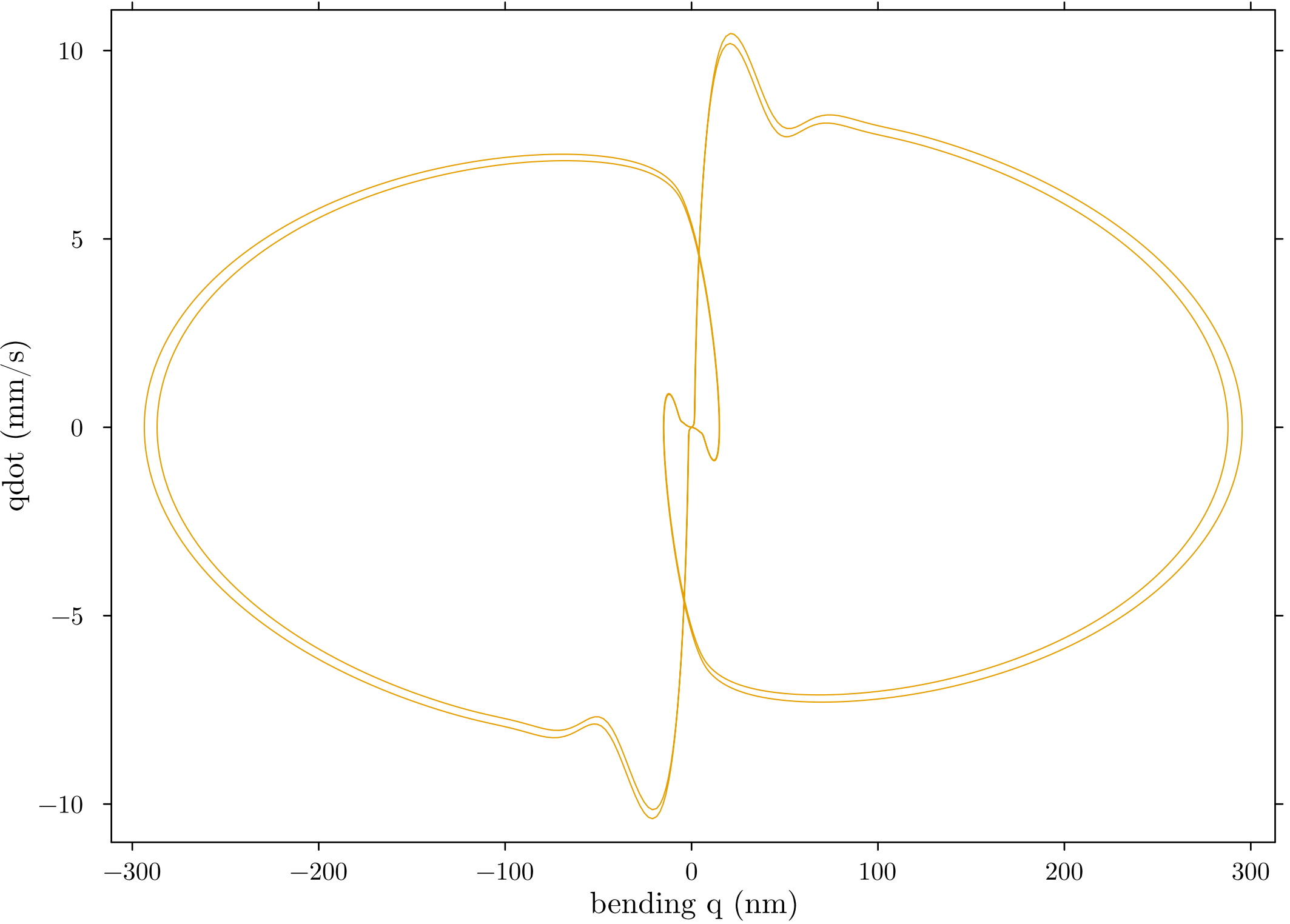
Electrode Bending Plane - last 2 cycles
