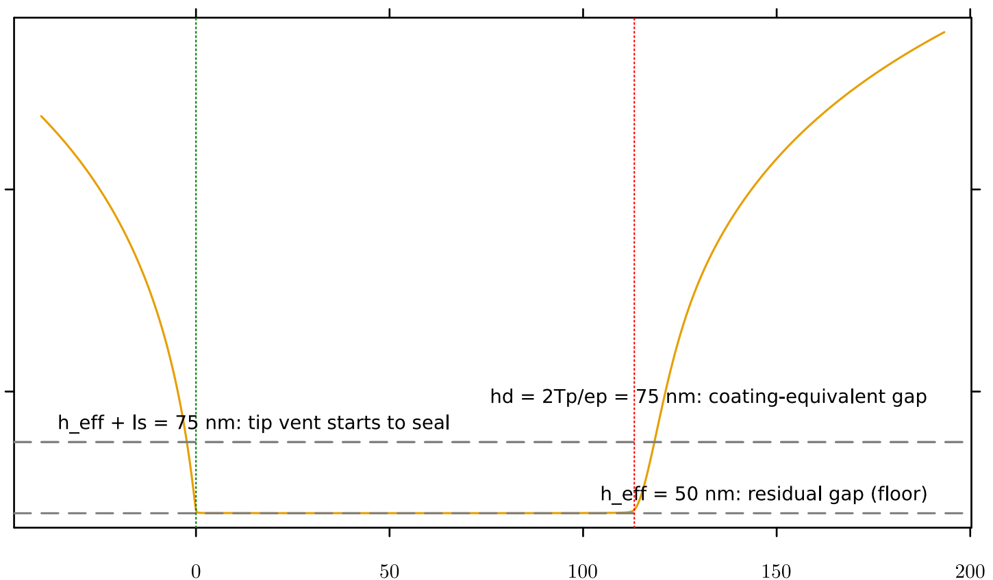
Bending of the compliant electrodes
