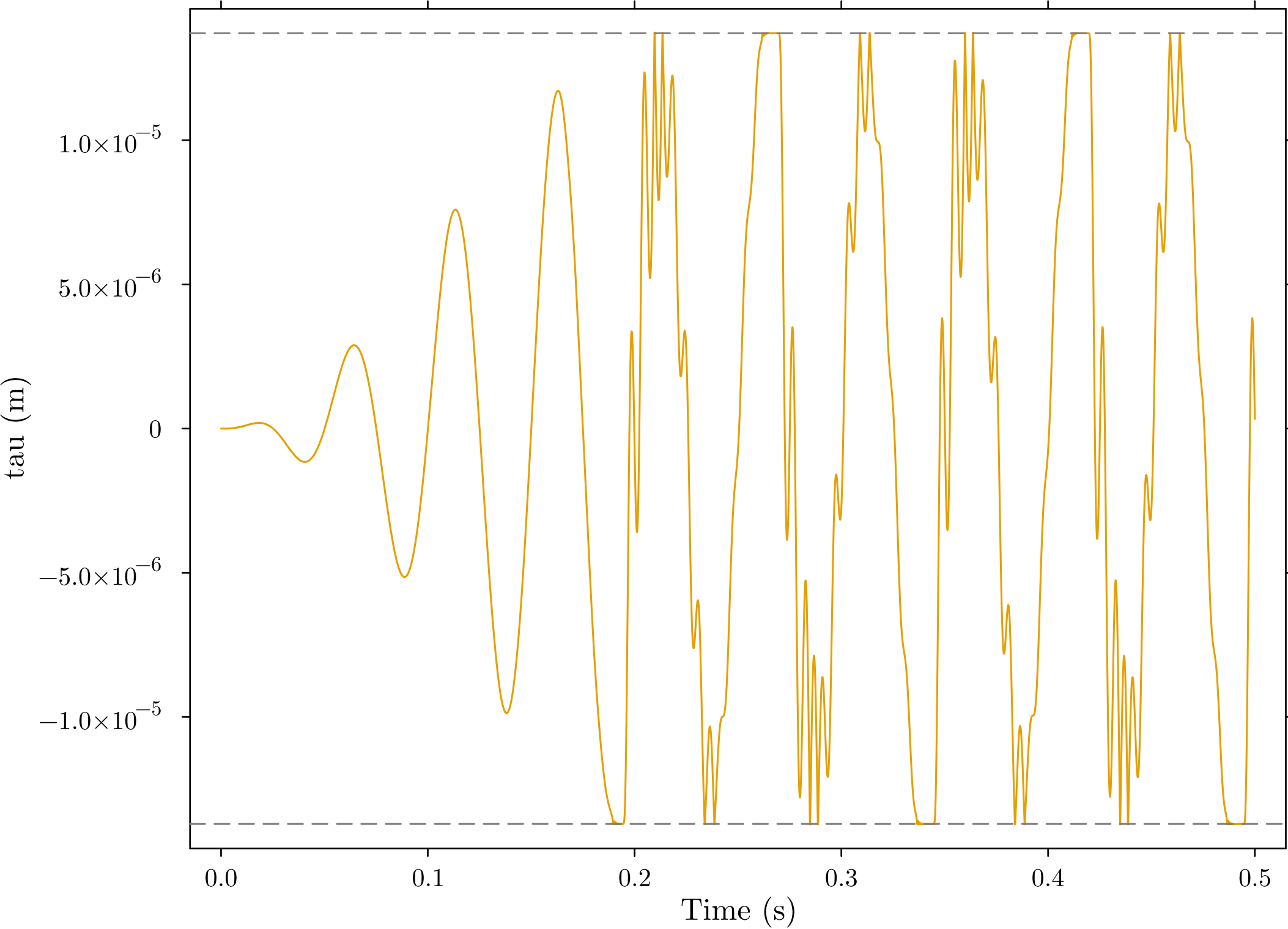
Compliant Tip Relative to its Stiff Face ( \tau )
