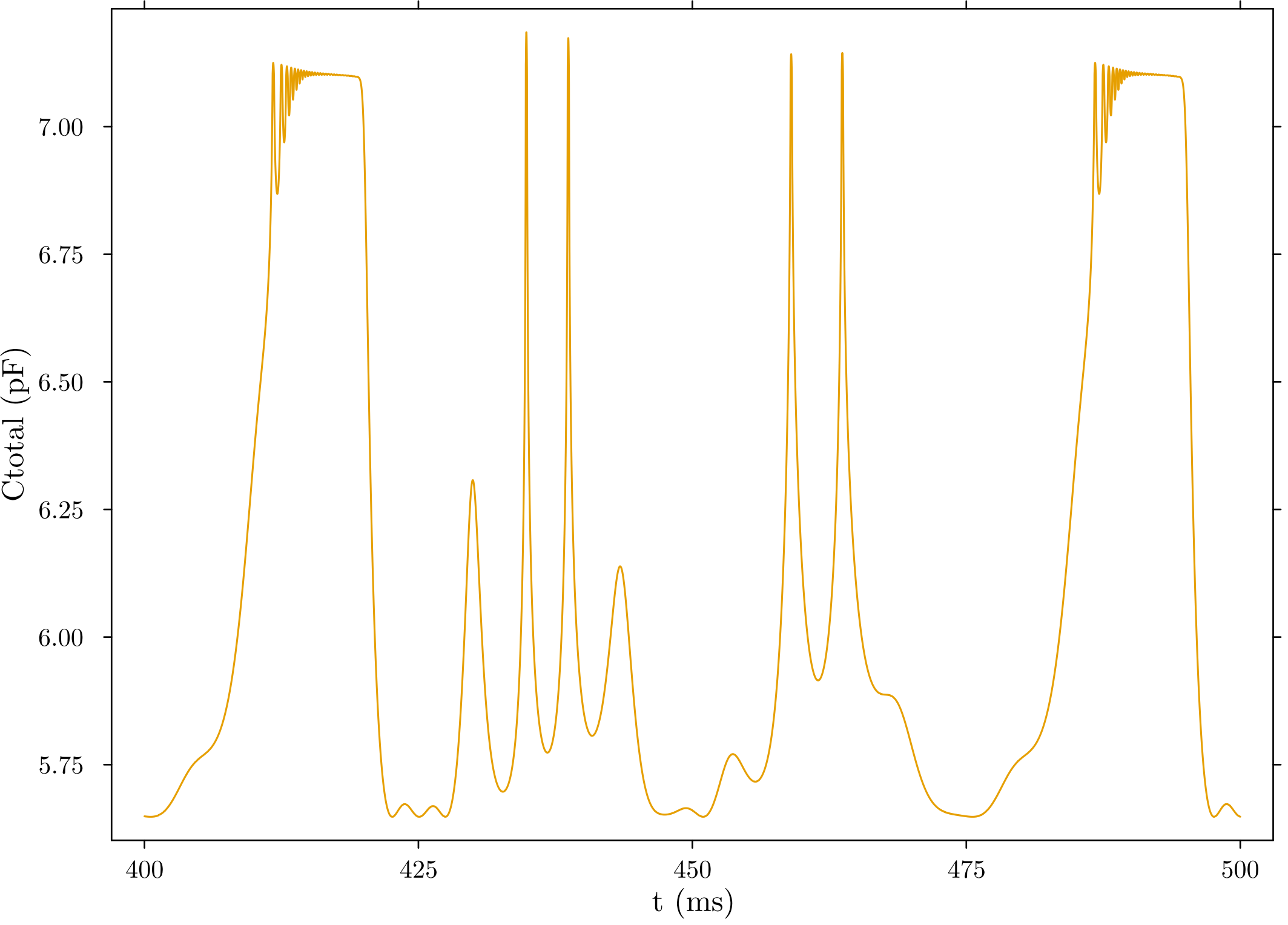
Total Capacitance - last 2 cycles
