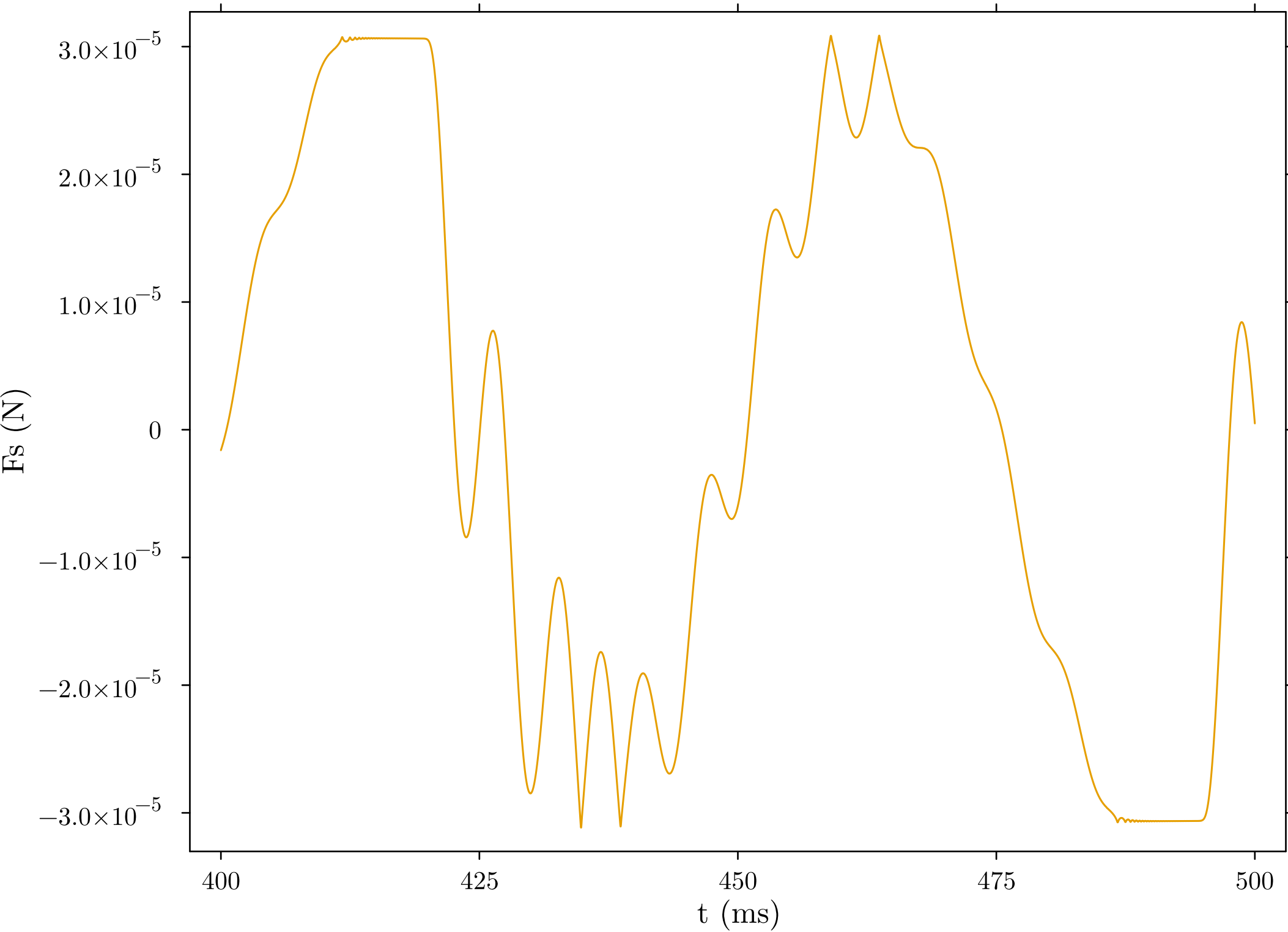
Suspension + Stopper Force on x1 - last 2 cycles
