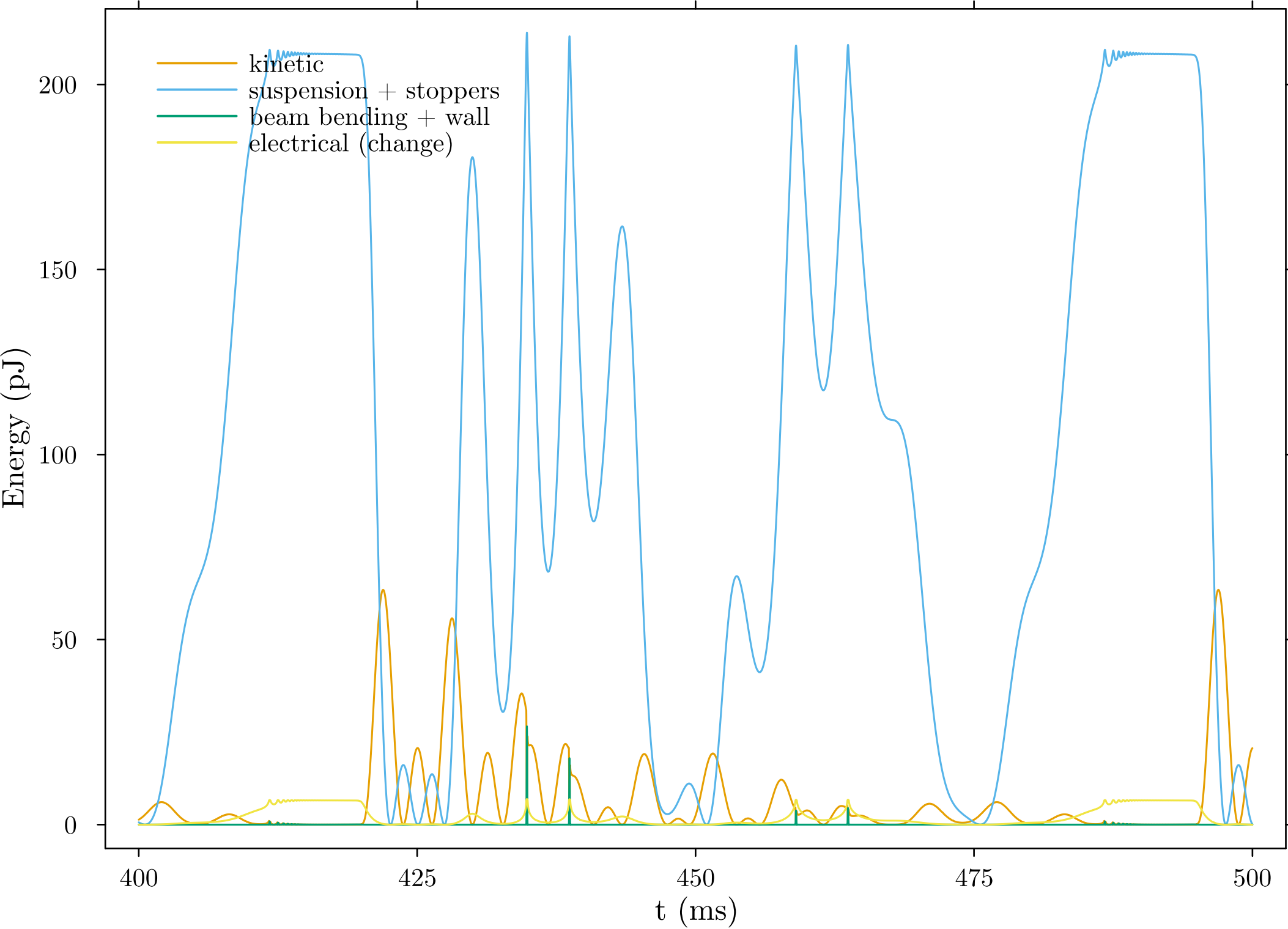
Stored Energy by Reservoir - last 2 cycles
