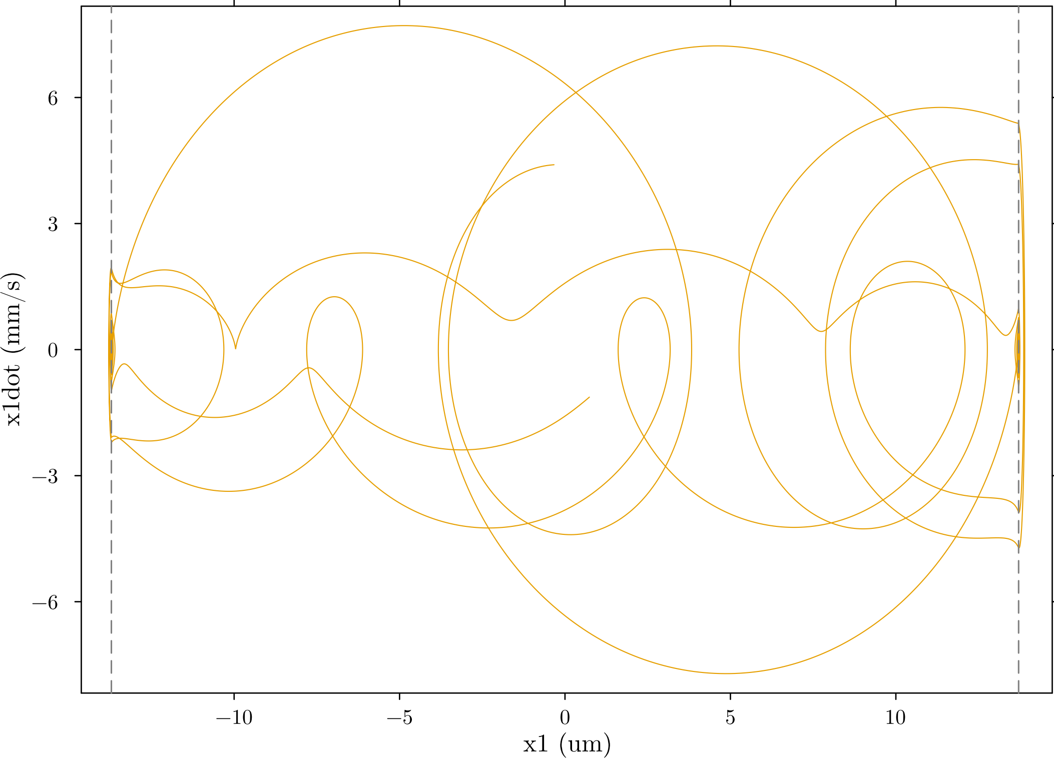
Shuttle Phase Plane - last 2 cycles
