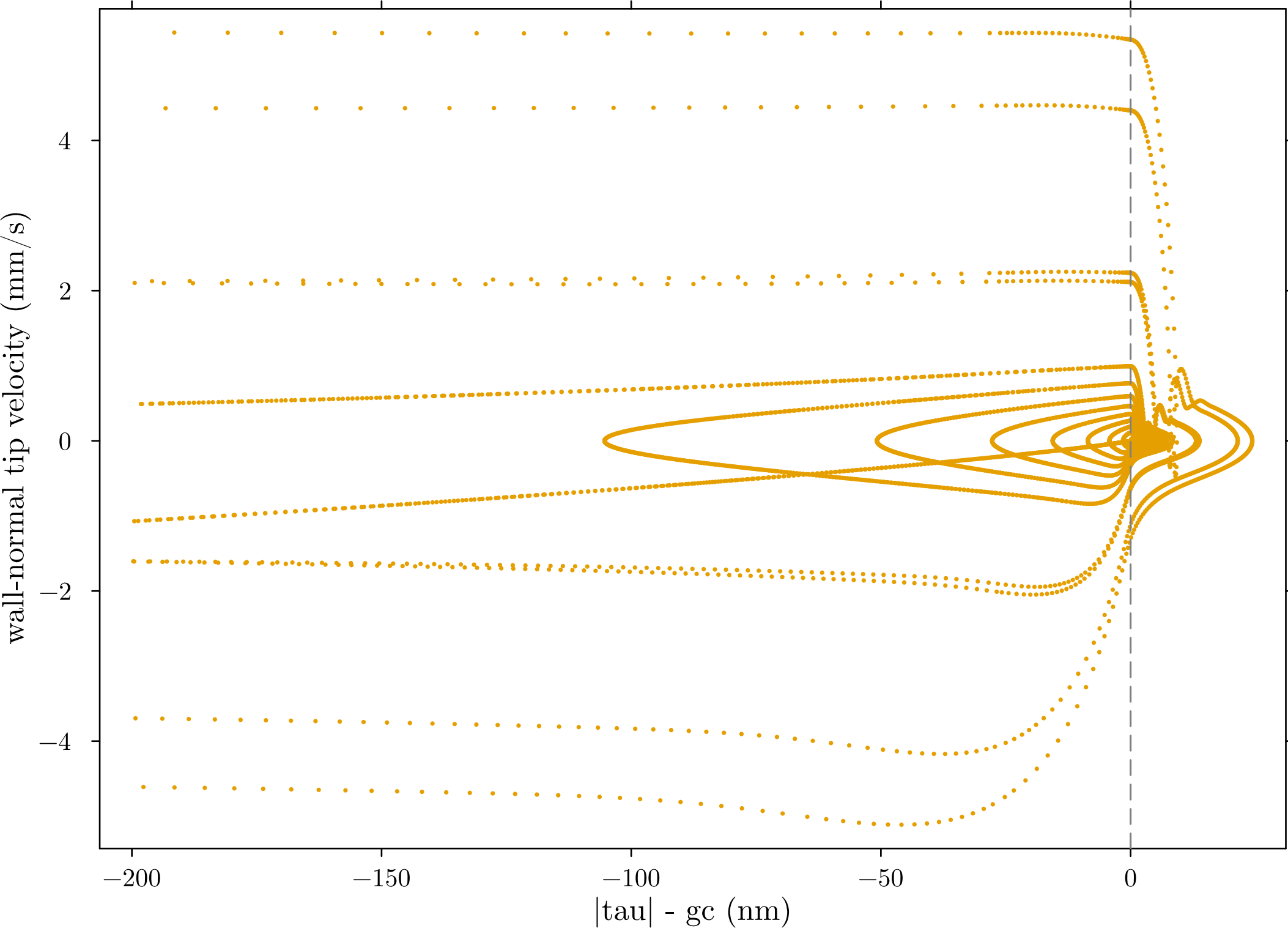
Phase Portrait at the Contact Boundary - last 2 cycles
