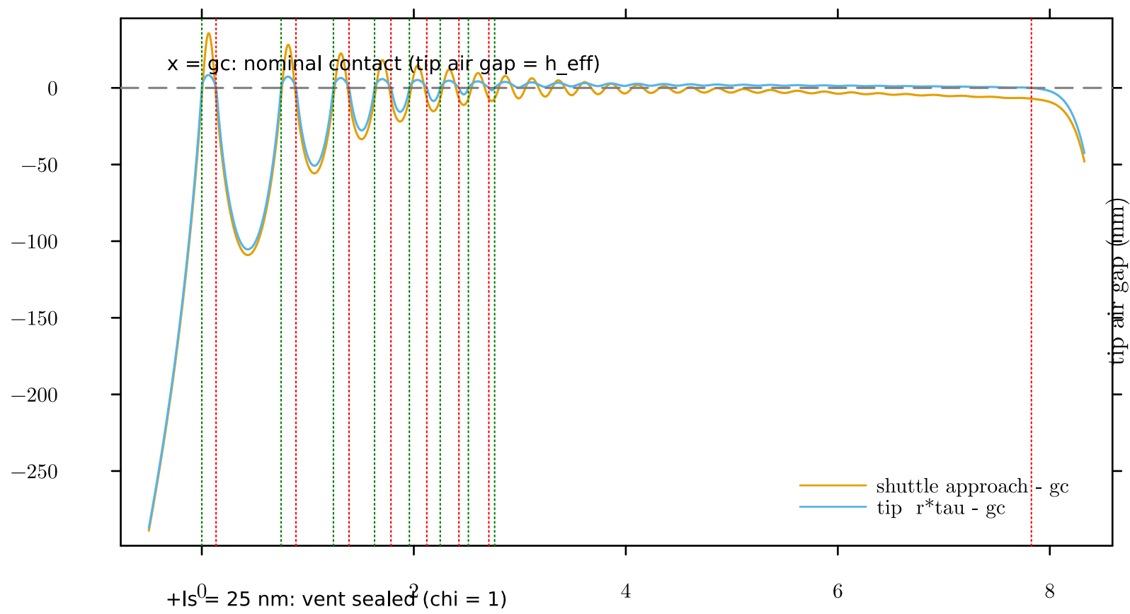
Nominal overlap and the tip-vent sealing window
