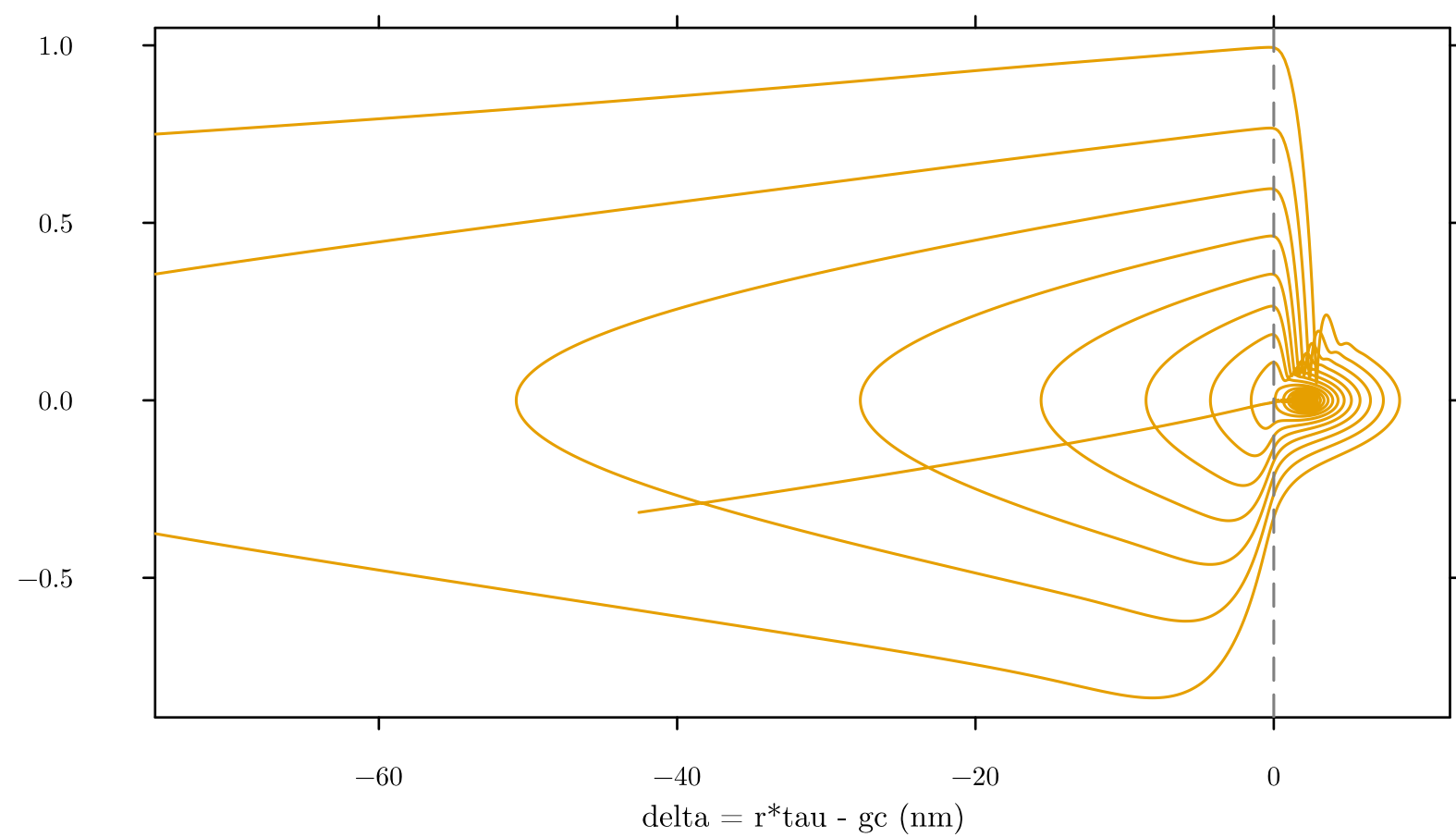
Phase portrait at the contact boundary
