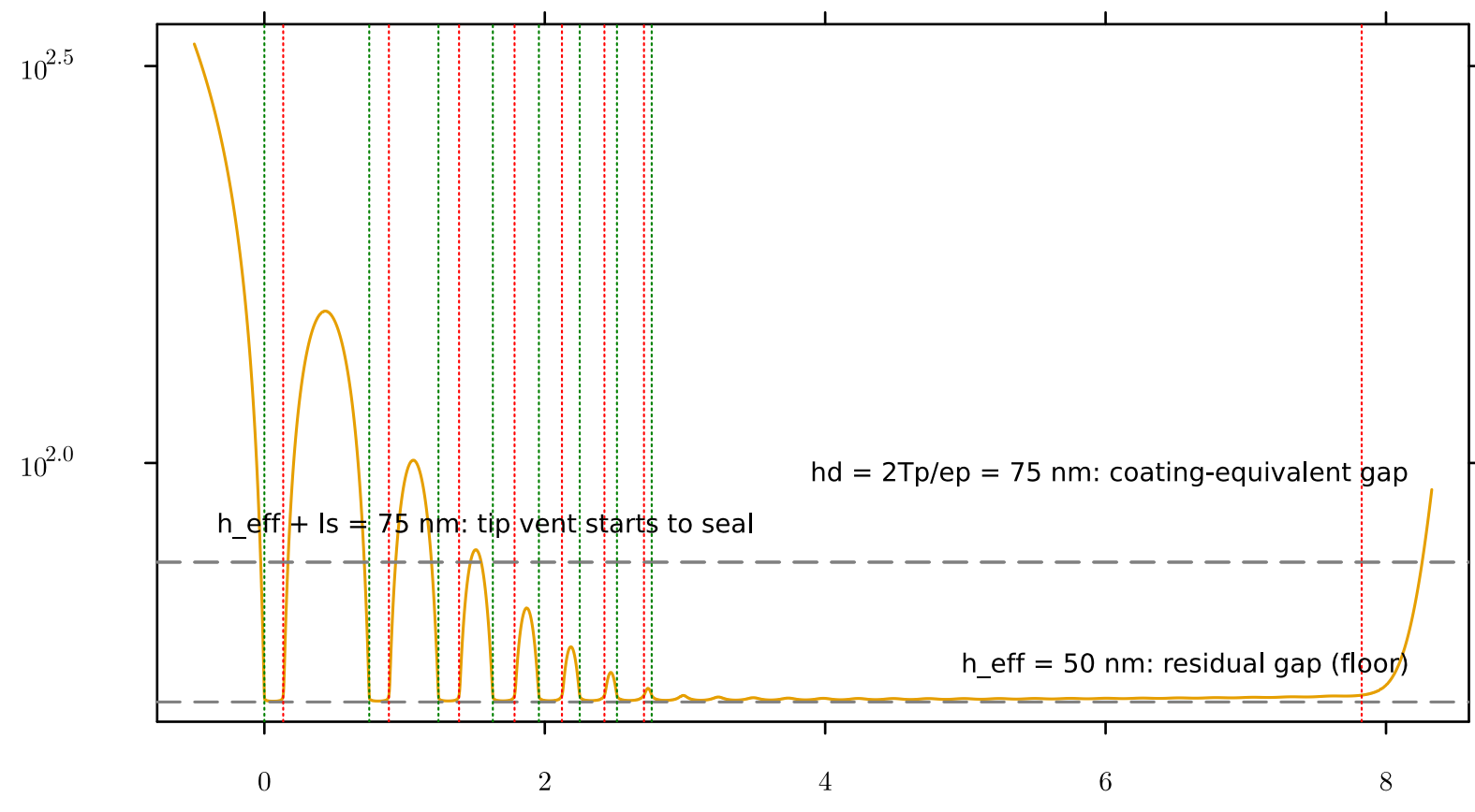
Bending of the compliant electrodes
