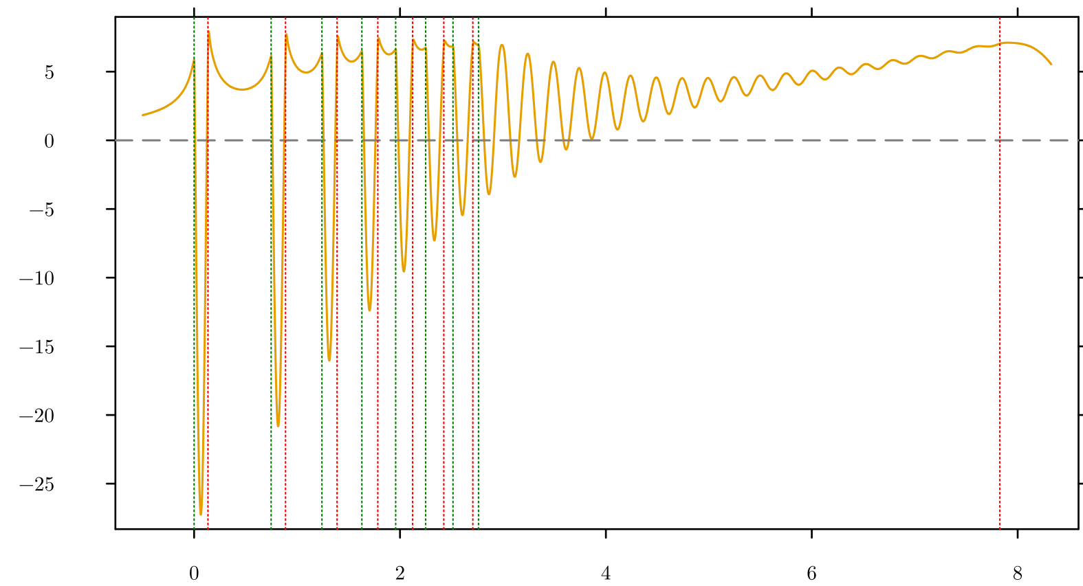
Forces on the tip coordinate (+ = into the wall)
