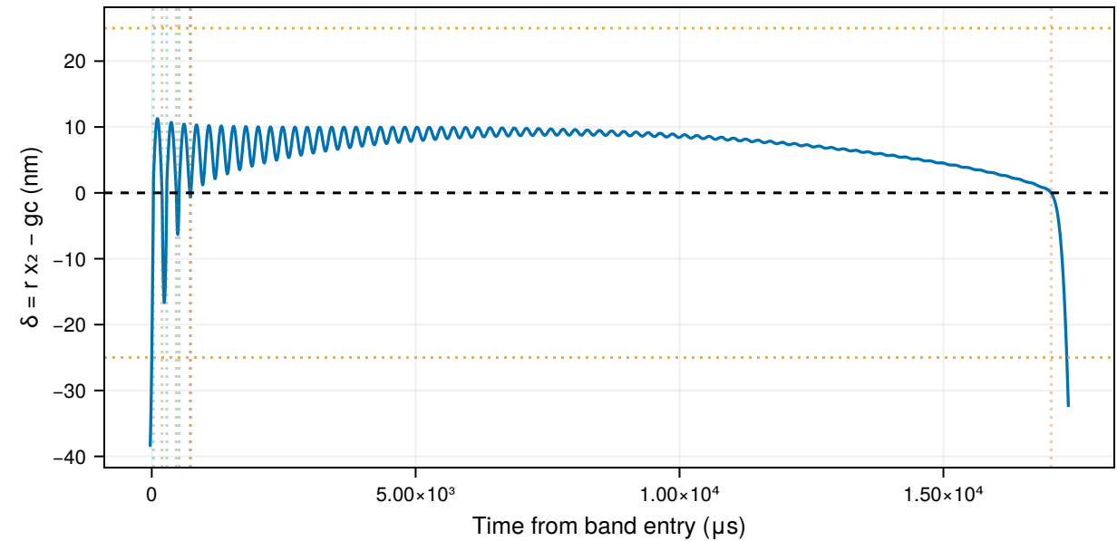
Nominal overlap \delta : full contact dwell
