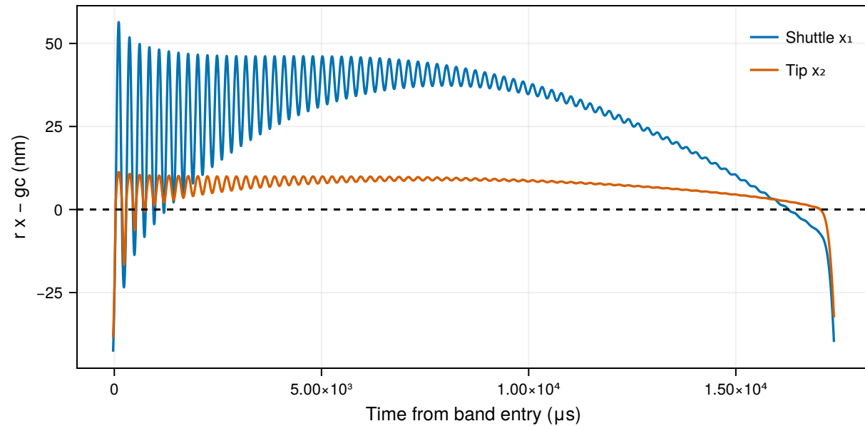
Shuttle and tip relative to the contact boundary
