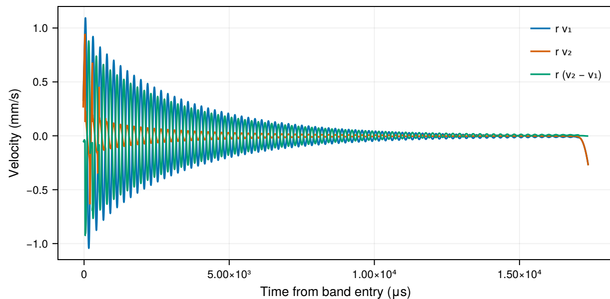
Velocities normal to this electrode
