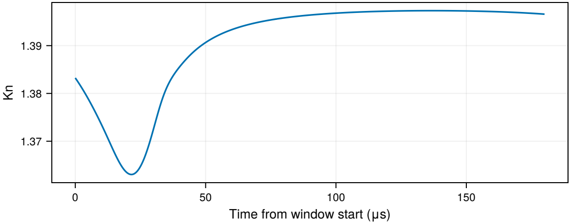
Maximum local Knudsen number
