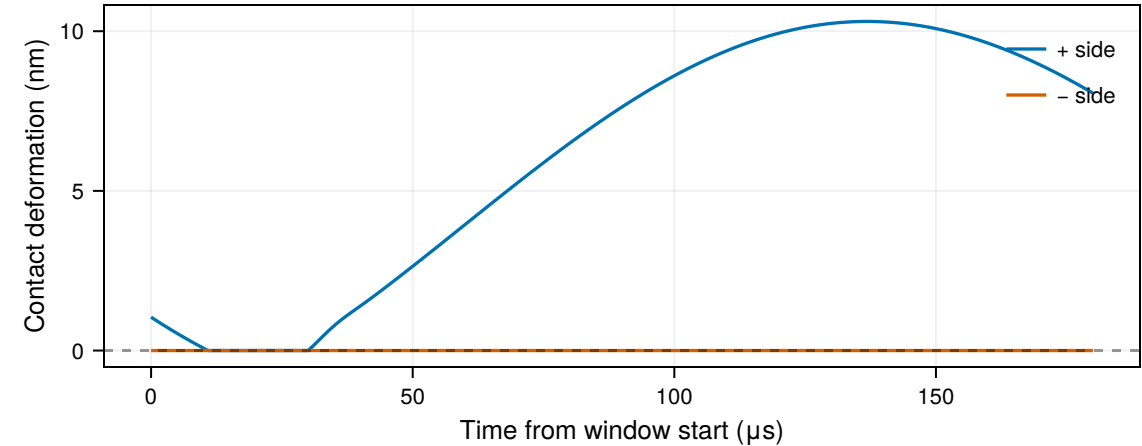
Positive nominal tip overlap
