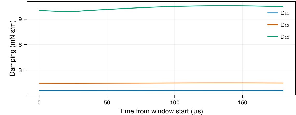
Fluid matrix entries
