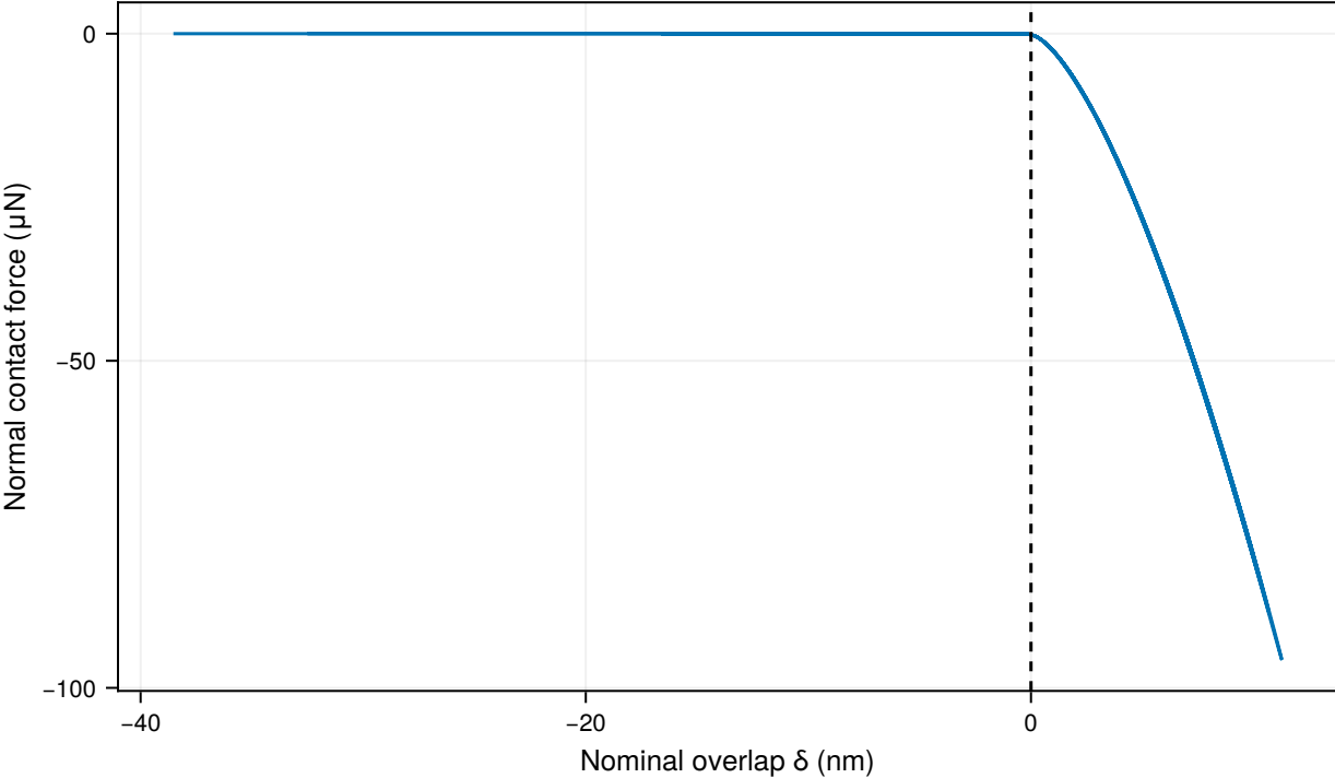
Realized contact force path
