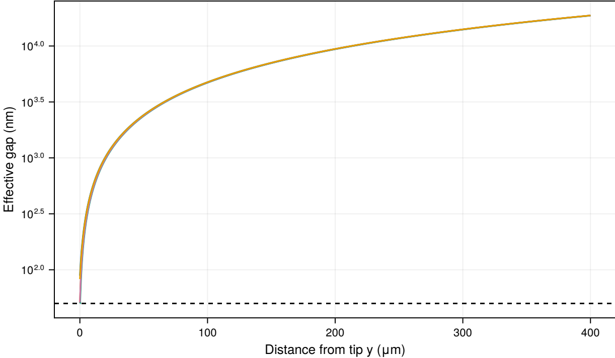
Effective gap along electrode
