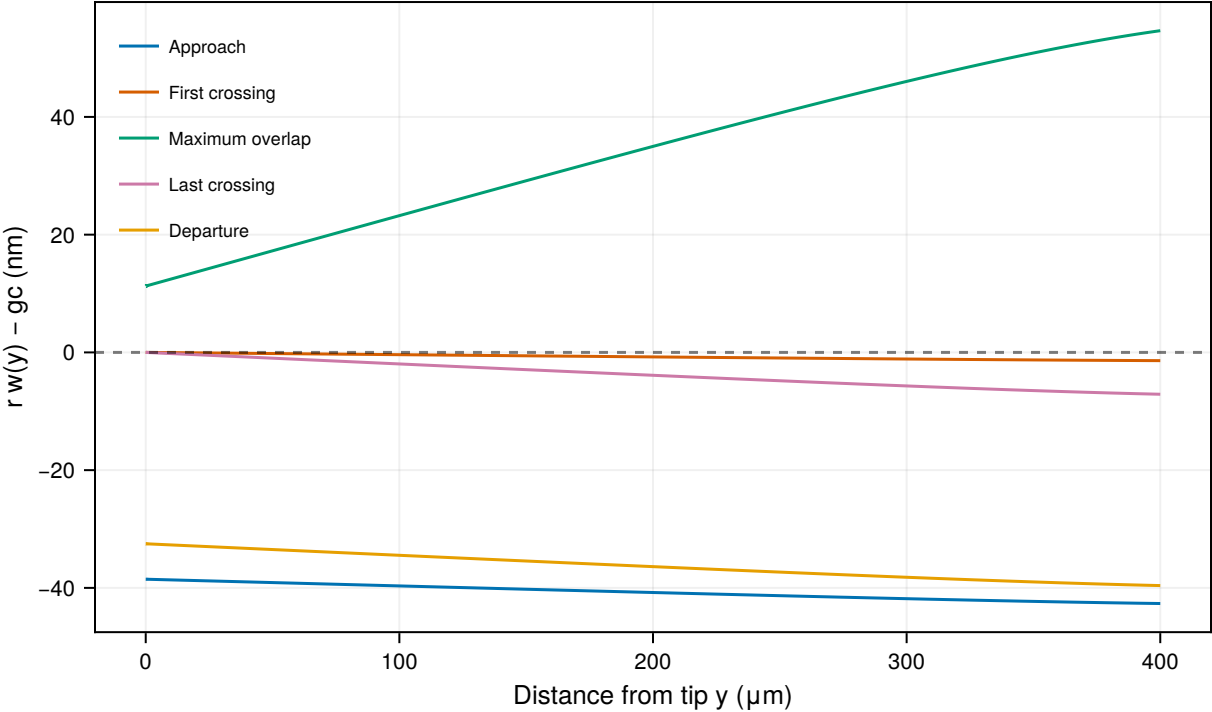
Reduced electrode displacement profile
