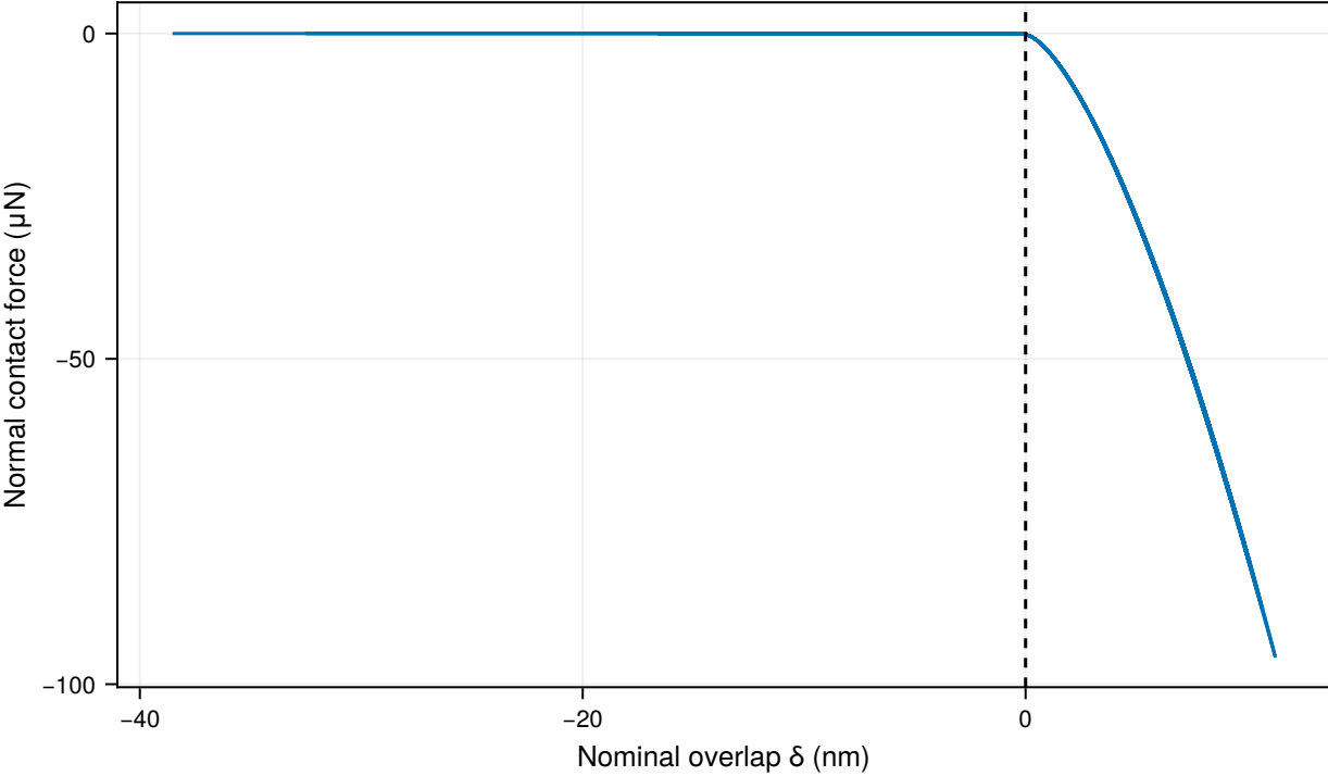
Realized contact force path
