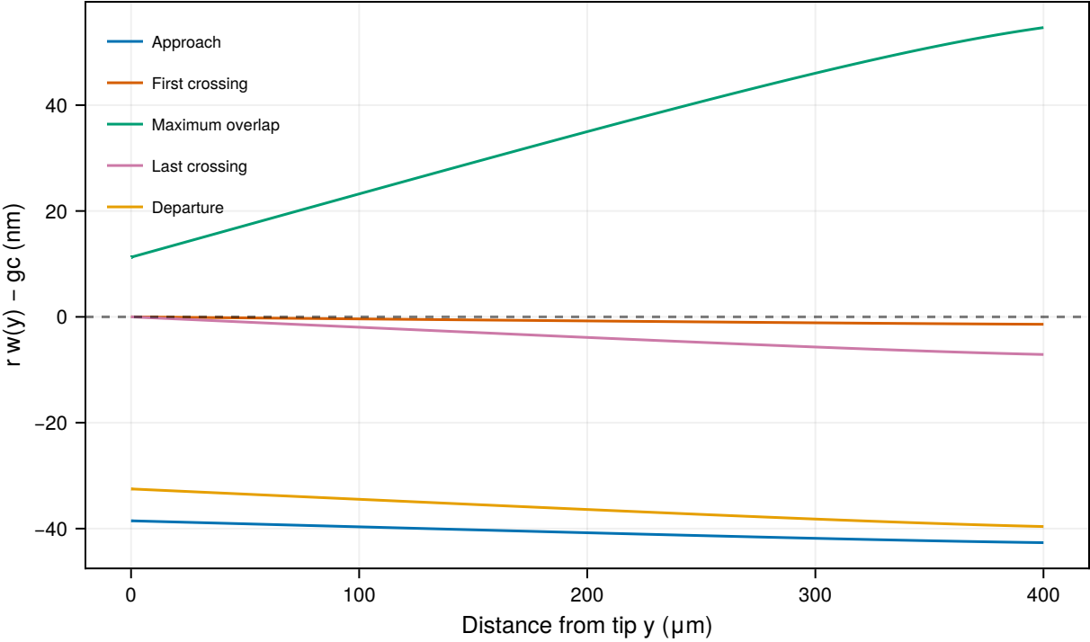
Tip-neighborhood gap
