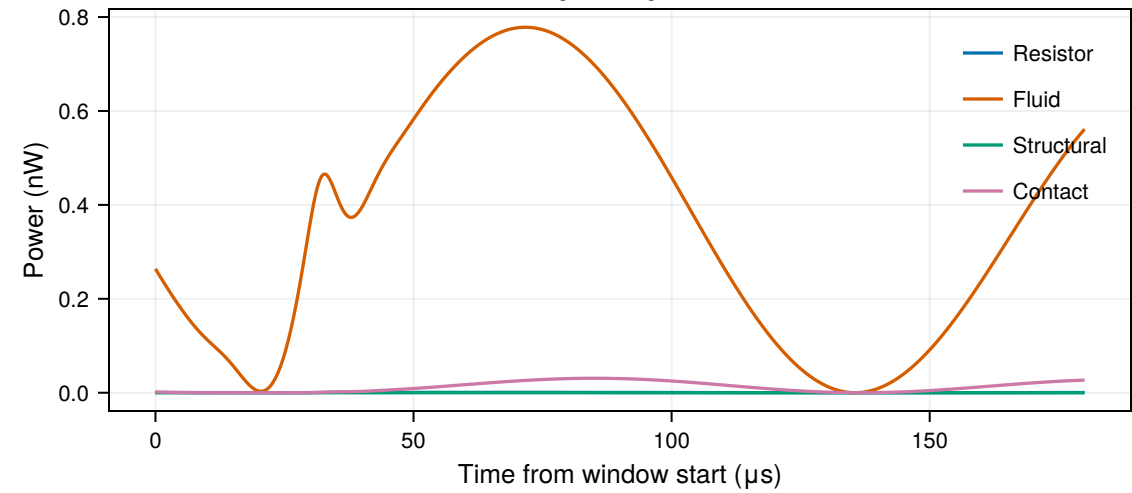
Energy-balance residual
