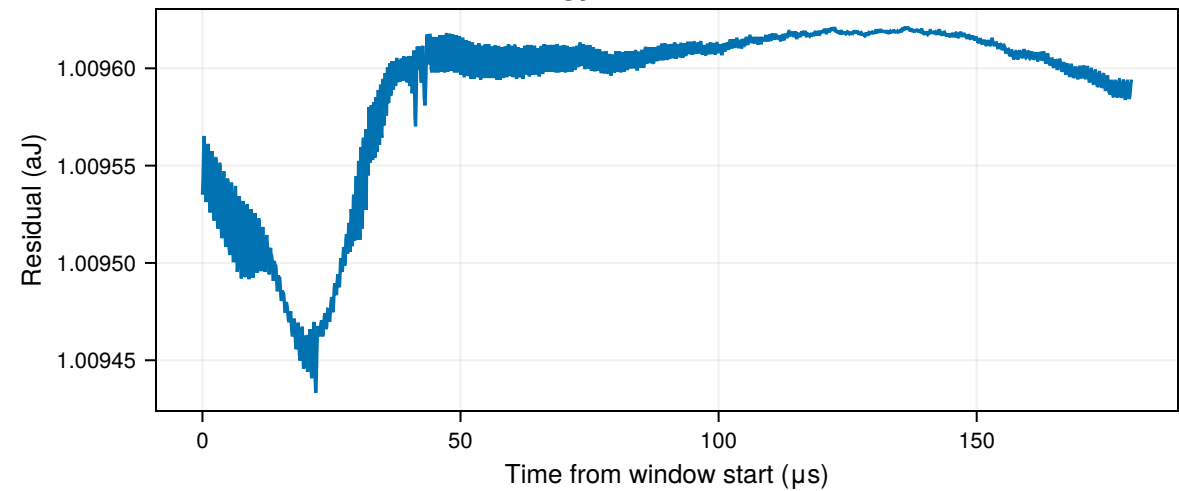
Energy-balance residual
