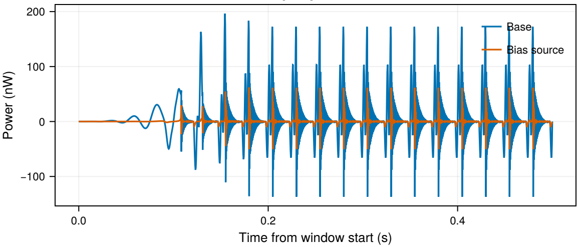
Input powers
