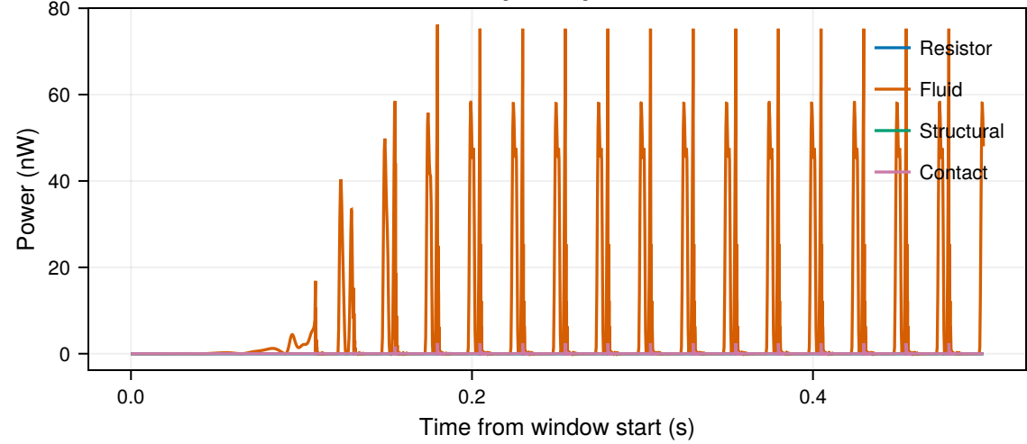
Dissipated powers
