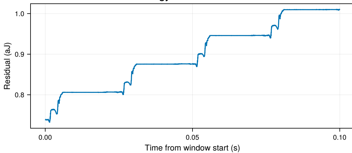
Energy-balance residual
