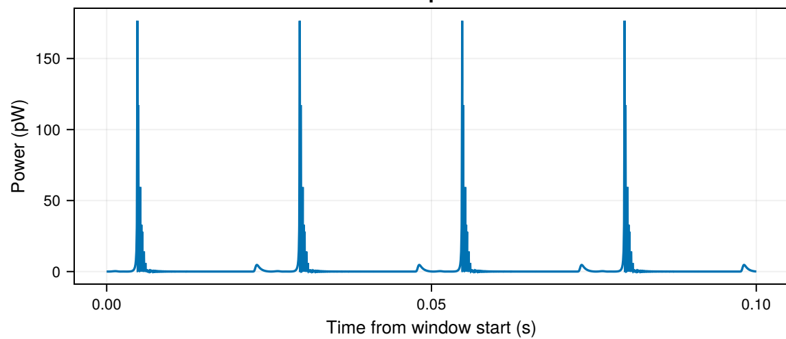
Load power
