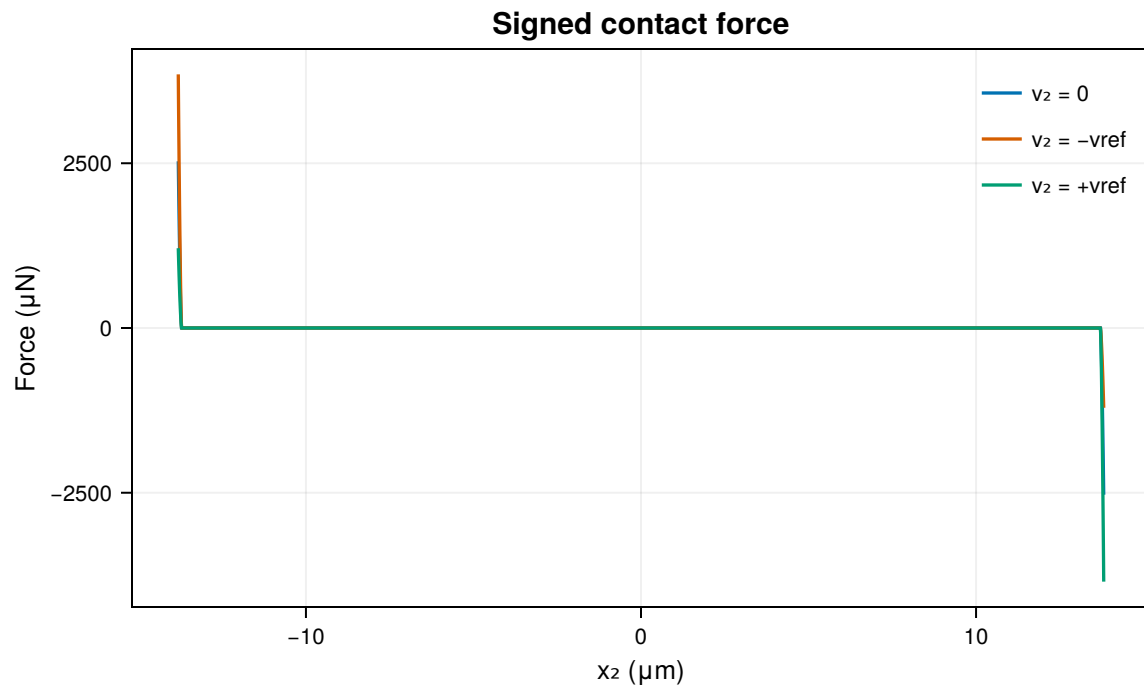
Contact force across both travel limits Full-device force on x_2 ; curves hold signed v_2 fixed at 0 and \pm 10.43 mm/s
