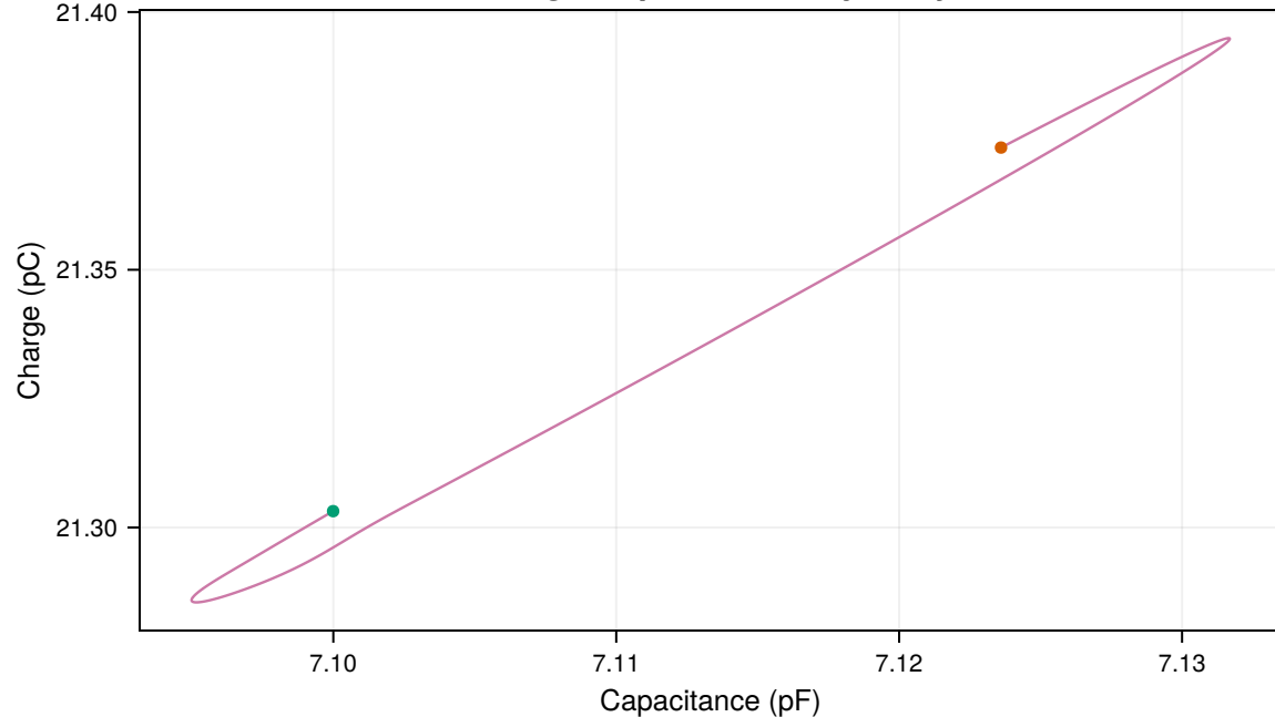
Charge-capacitance trajectory
