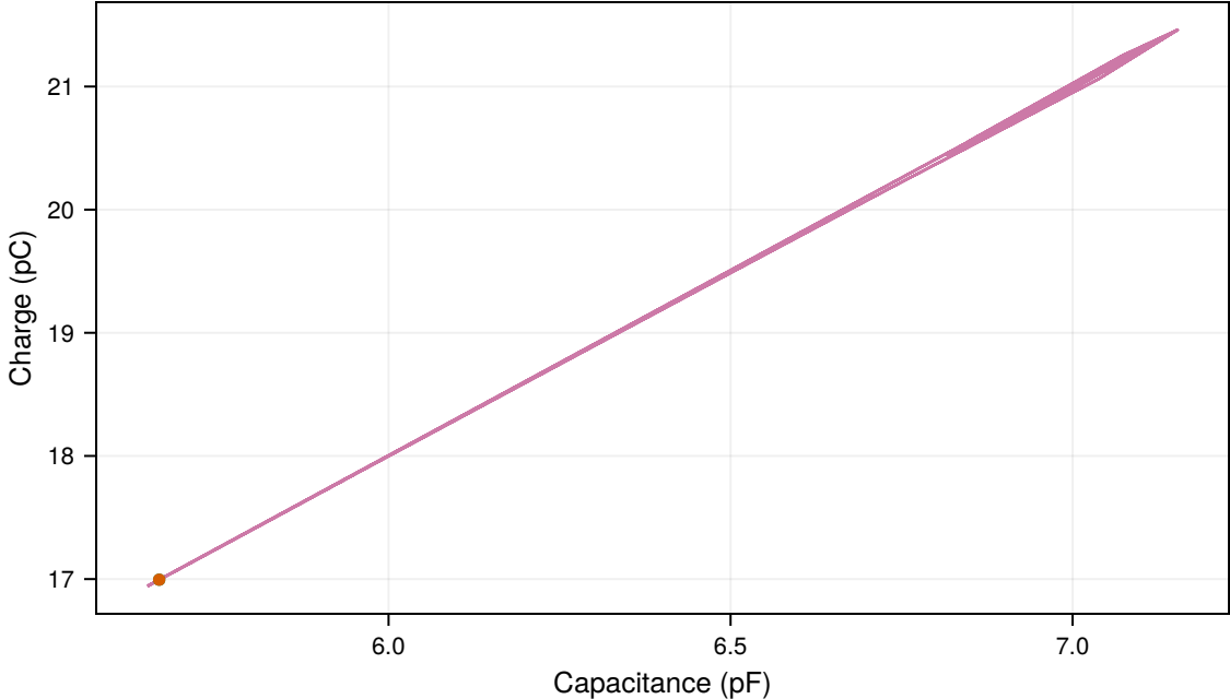
Charge–capacitance trajectory
