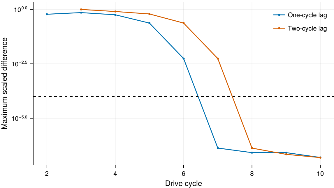
Period-1 and period-2 recurrence
