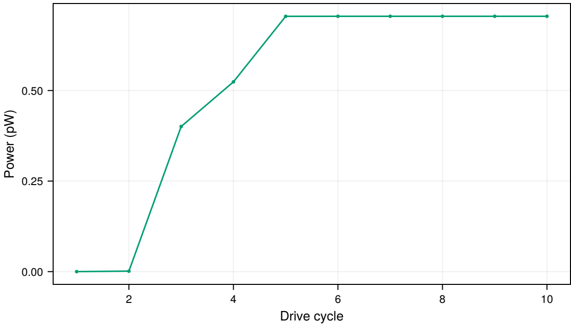
Mean resistor power per drive cycle
