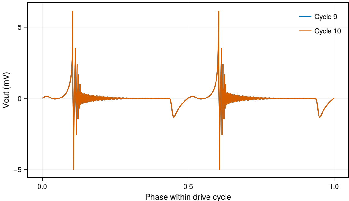
Last two voltage waveforms
