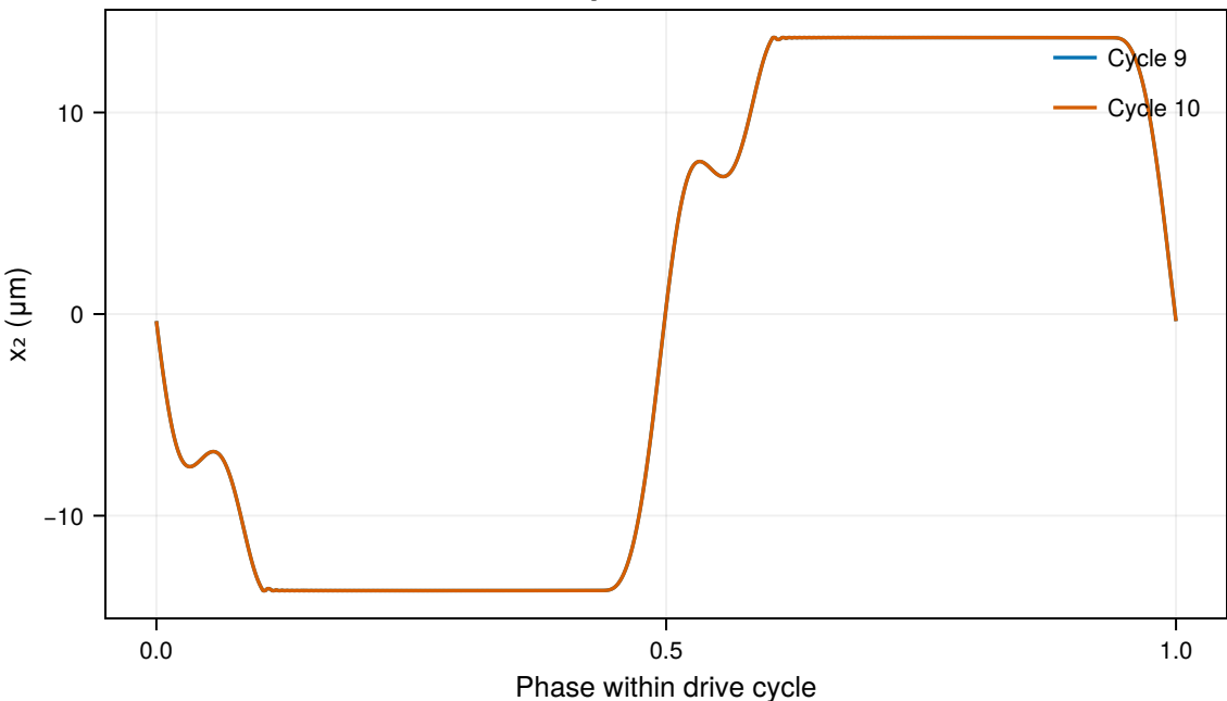
Last two displacement waveforms
