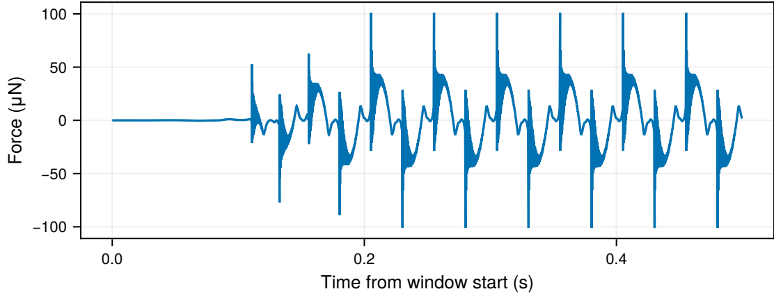
Electrode bending
