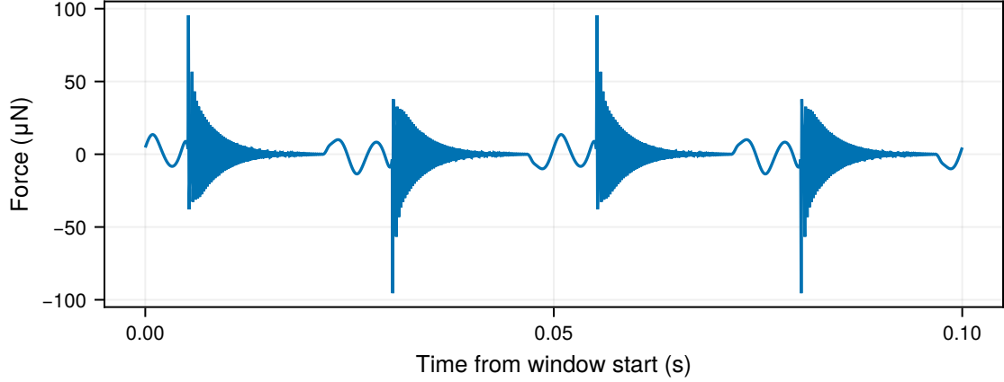
Net applied
