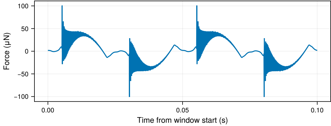
Electrode bending
