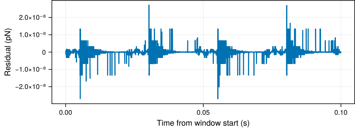
Force-balance residual
