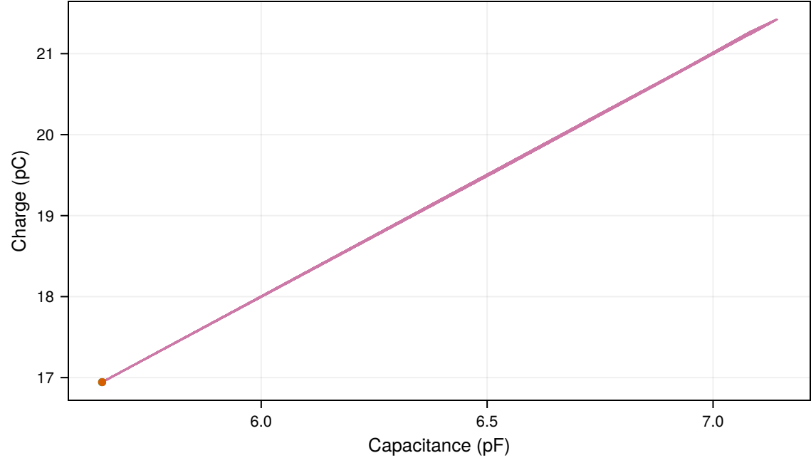
Charge-capacitance trajectory
