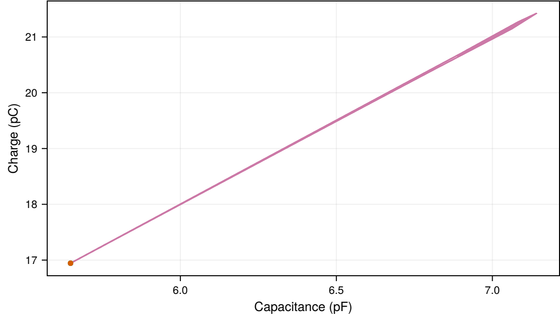
Charge-capacitance trajectory
