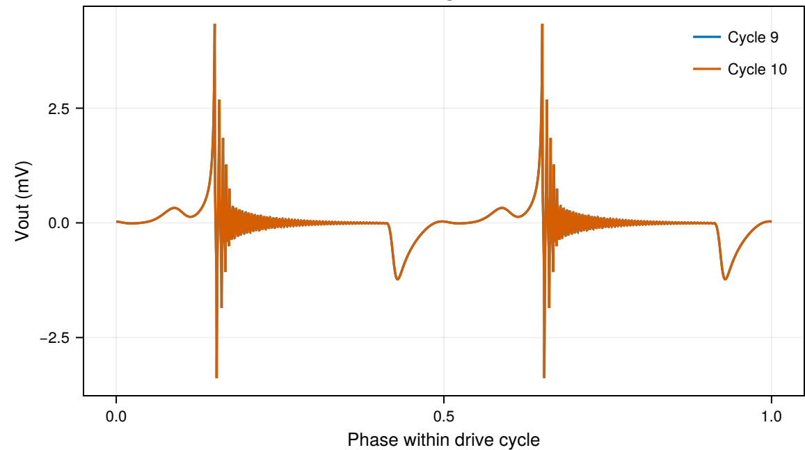
Last two voltage waveforms
