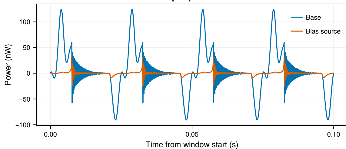
Load power
