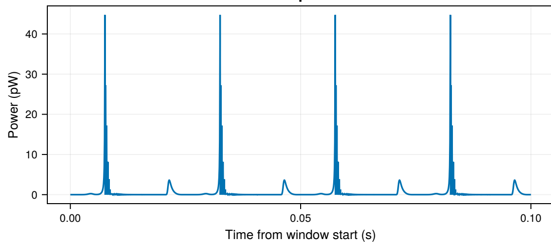
Load power
