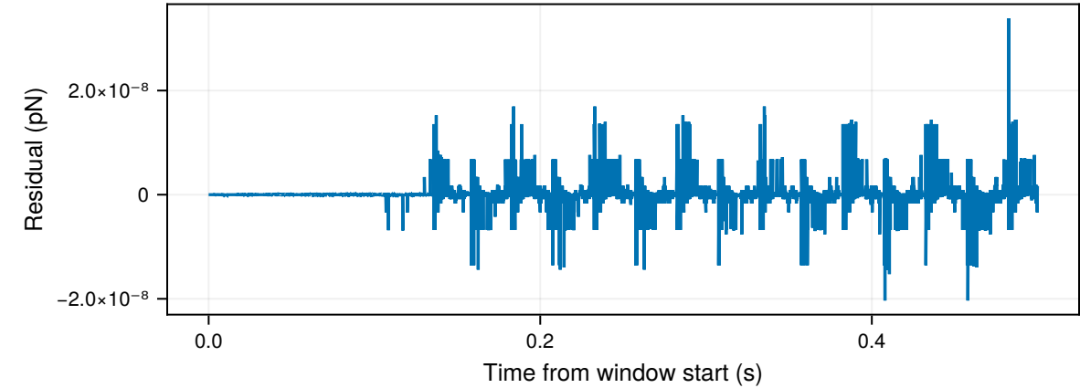
Force-balance residual
