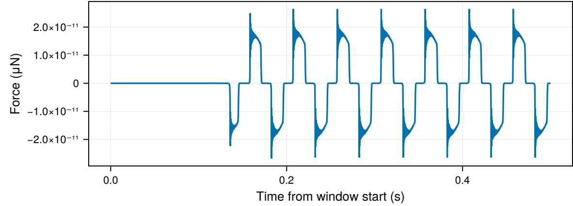
Soft stopper
