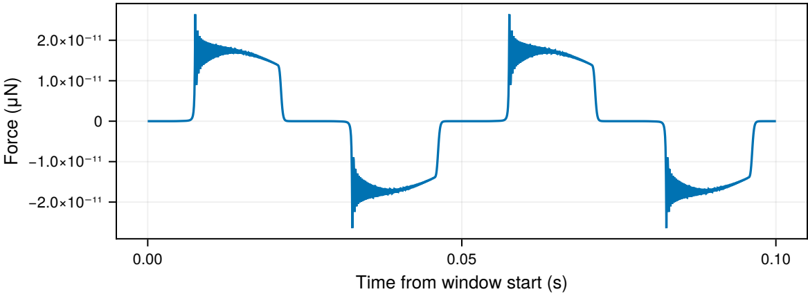
Soft stopper
