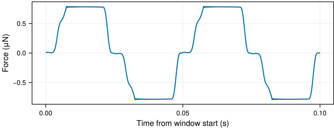
Suspension: cubic
