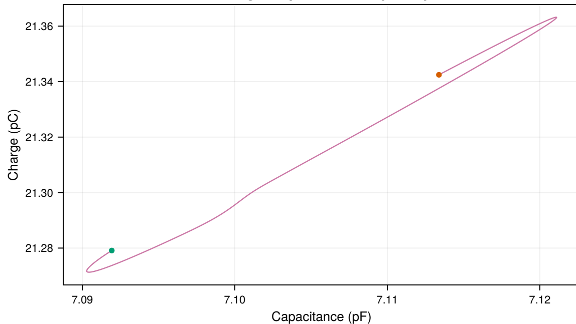
Charge-capacitance trajectory
