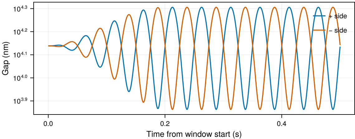
Minimum effective gap along electrode
