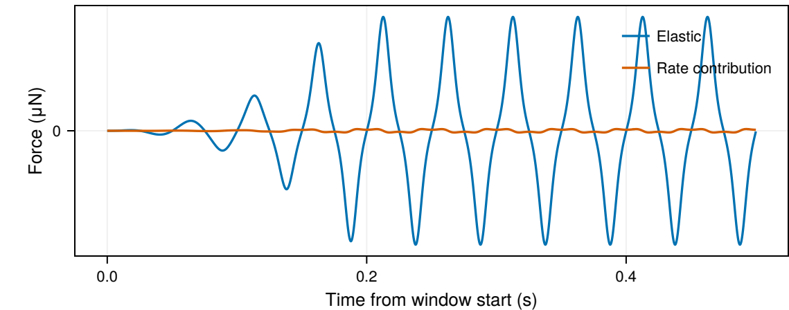
Contact-force decomposition on x_2
