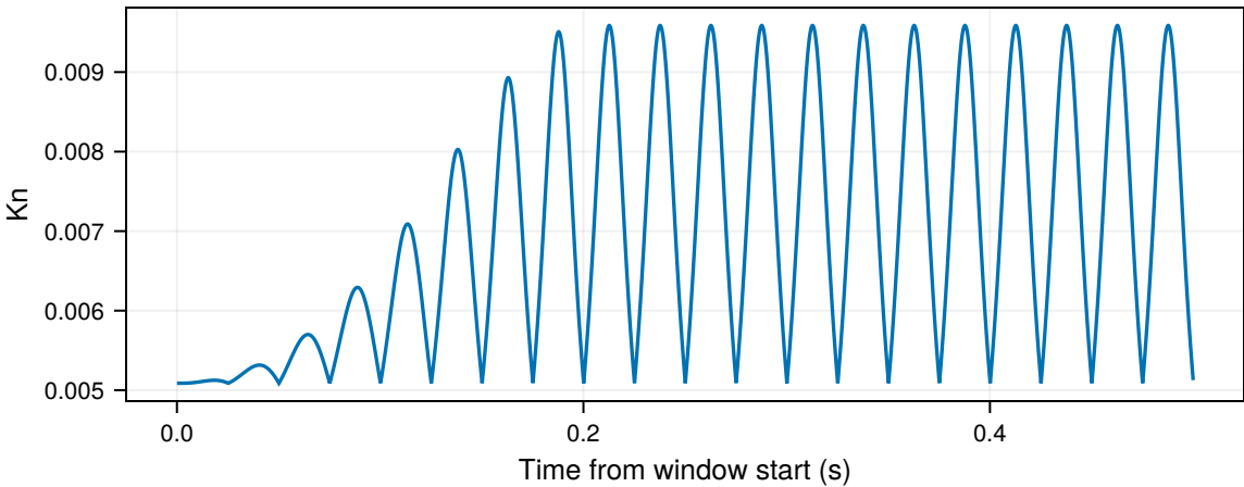
Maximum local Knudsen number
