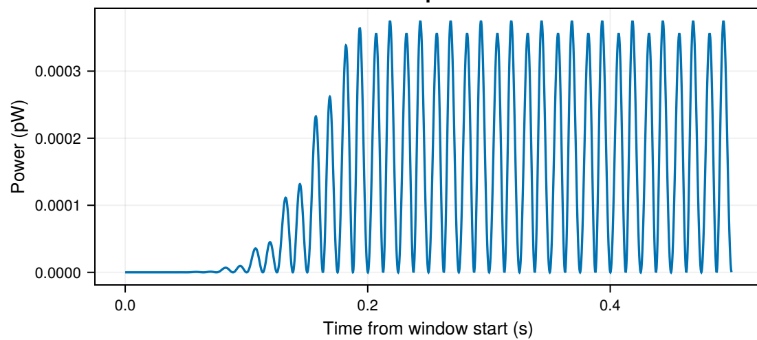
Load power
