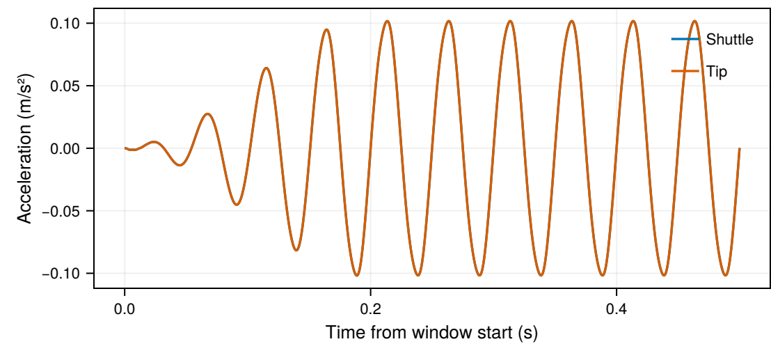
Mechanical accelerations
