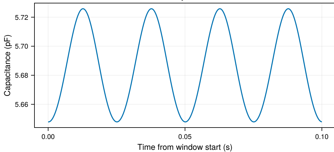
Total capacitance
