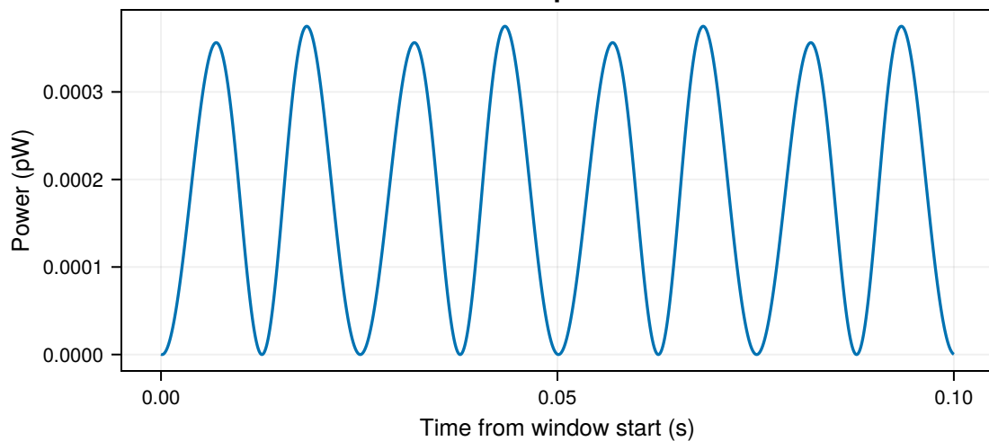
Load power
