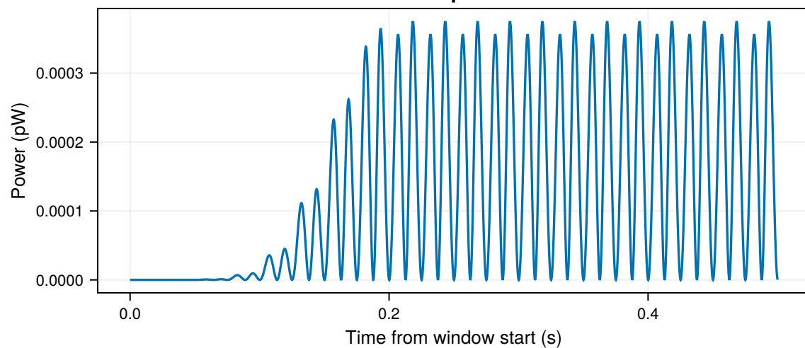
Load power
