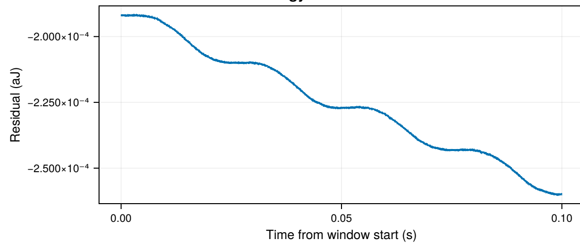
Energy-balance residual
