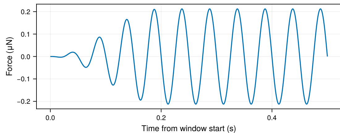
Force-balance residual
