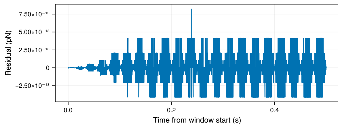
Force-balance residual
