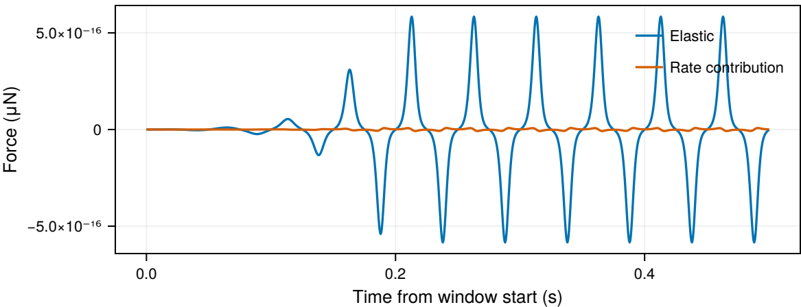
Contact-force decomposition on x_2
