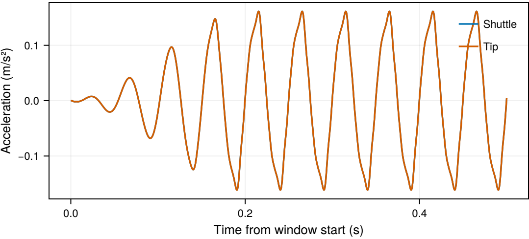
Mechanical accelerations
