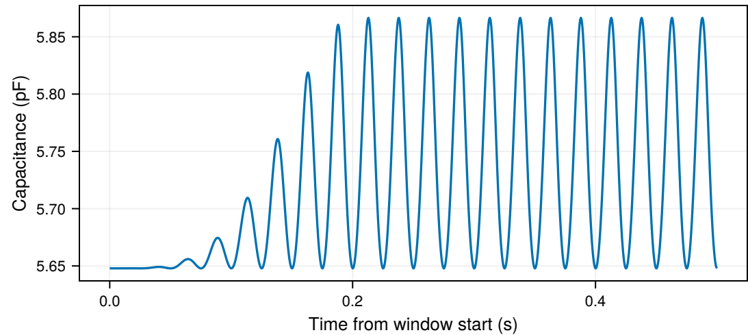
Total capacitance
