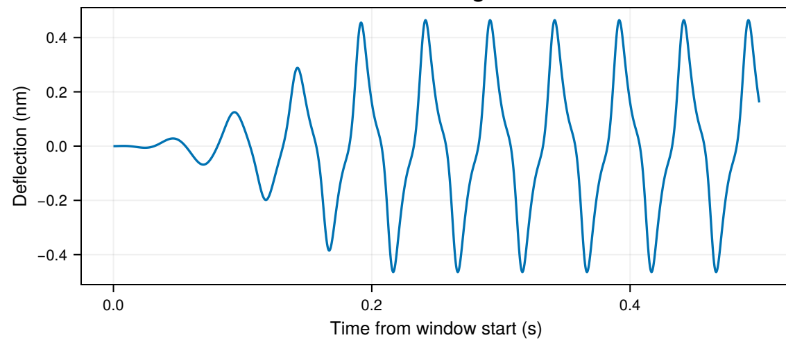
Relative bending x_2 - x_1
