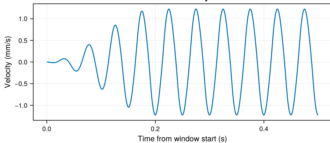
Shuttle velocity v_1
