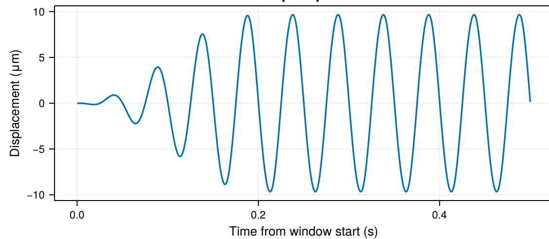
Electrode-tip displacement x_2
