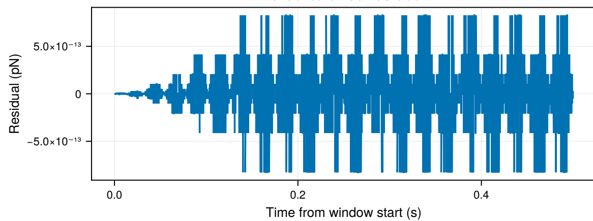
Force-balance residual
