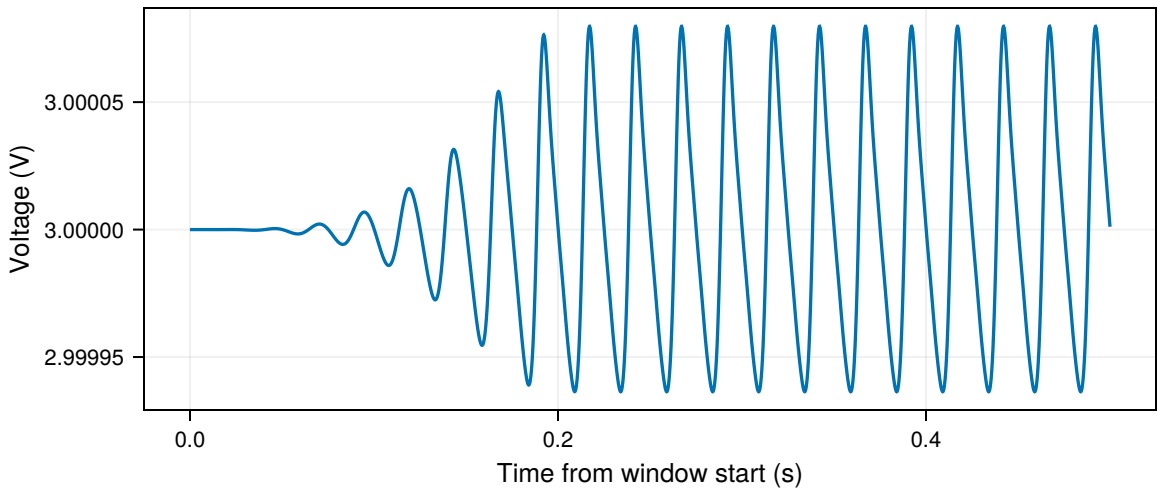
Capacitor voltage
