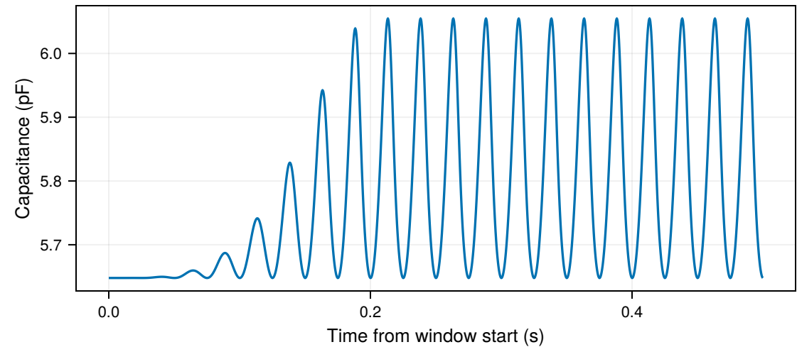
Total capacitance
