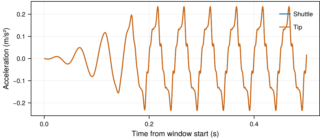
Mechanical accelerations
