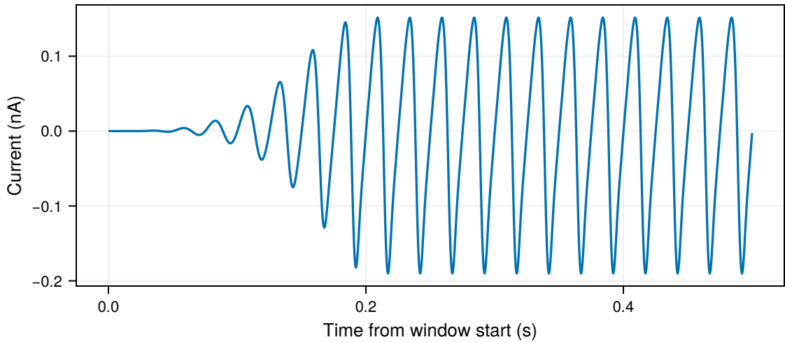
Load current
