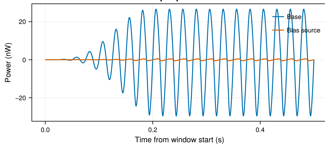
Load power
