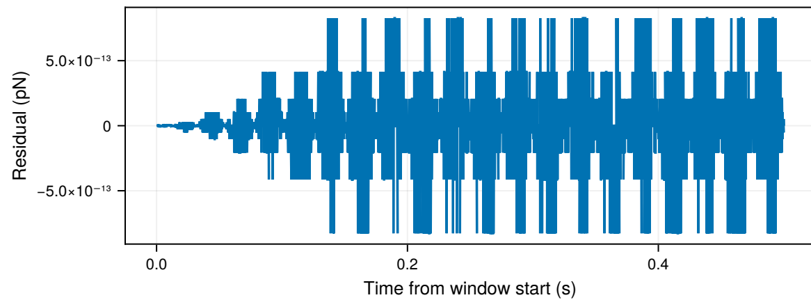
Force-balance residual
