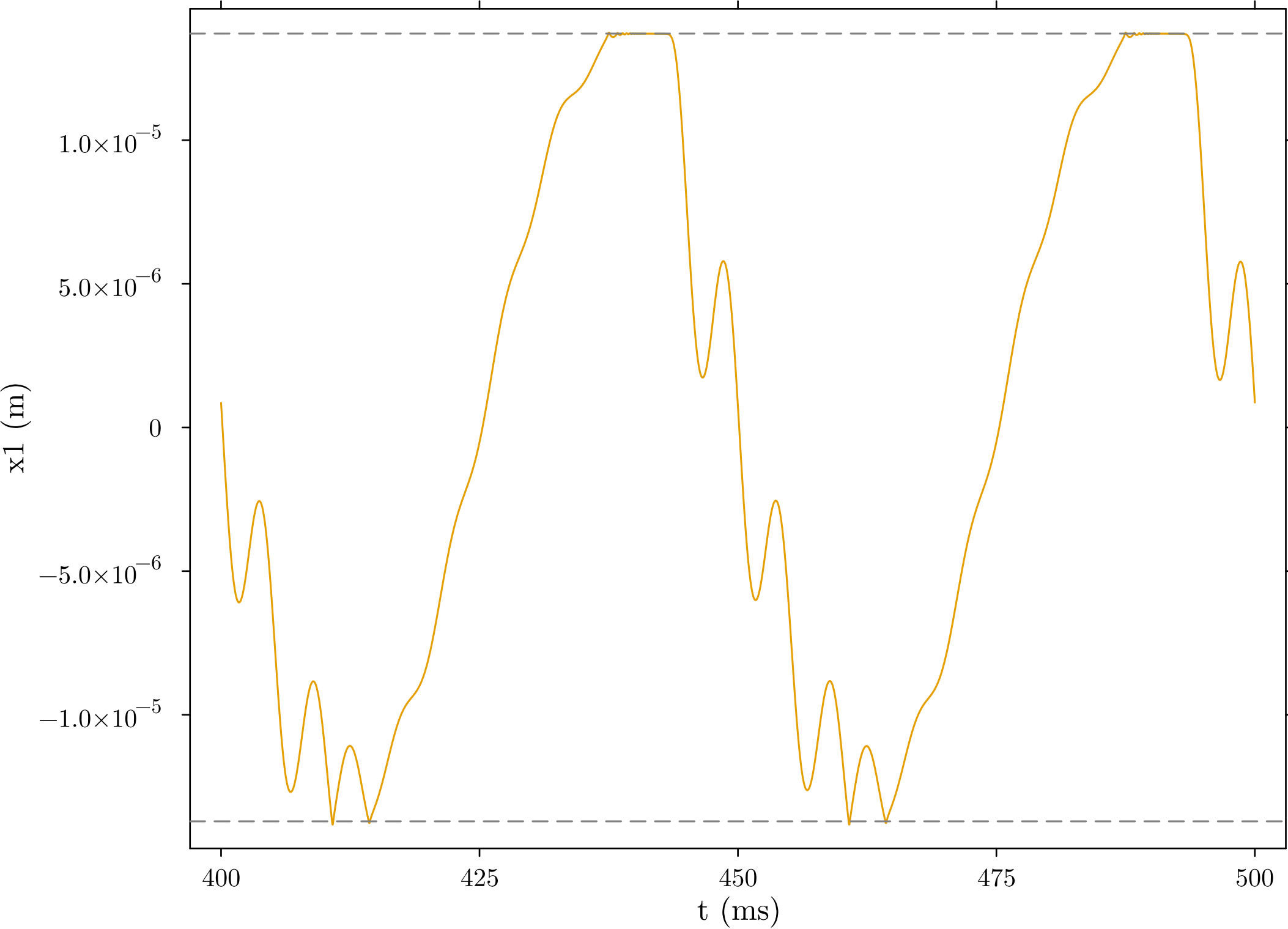
Shuttle Mass Displacement (x1) - last 2 cycles
