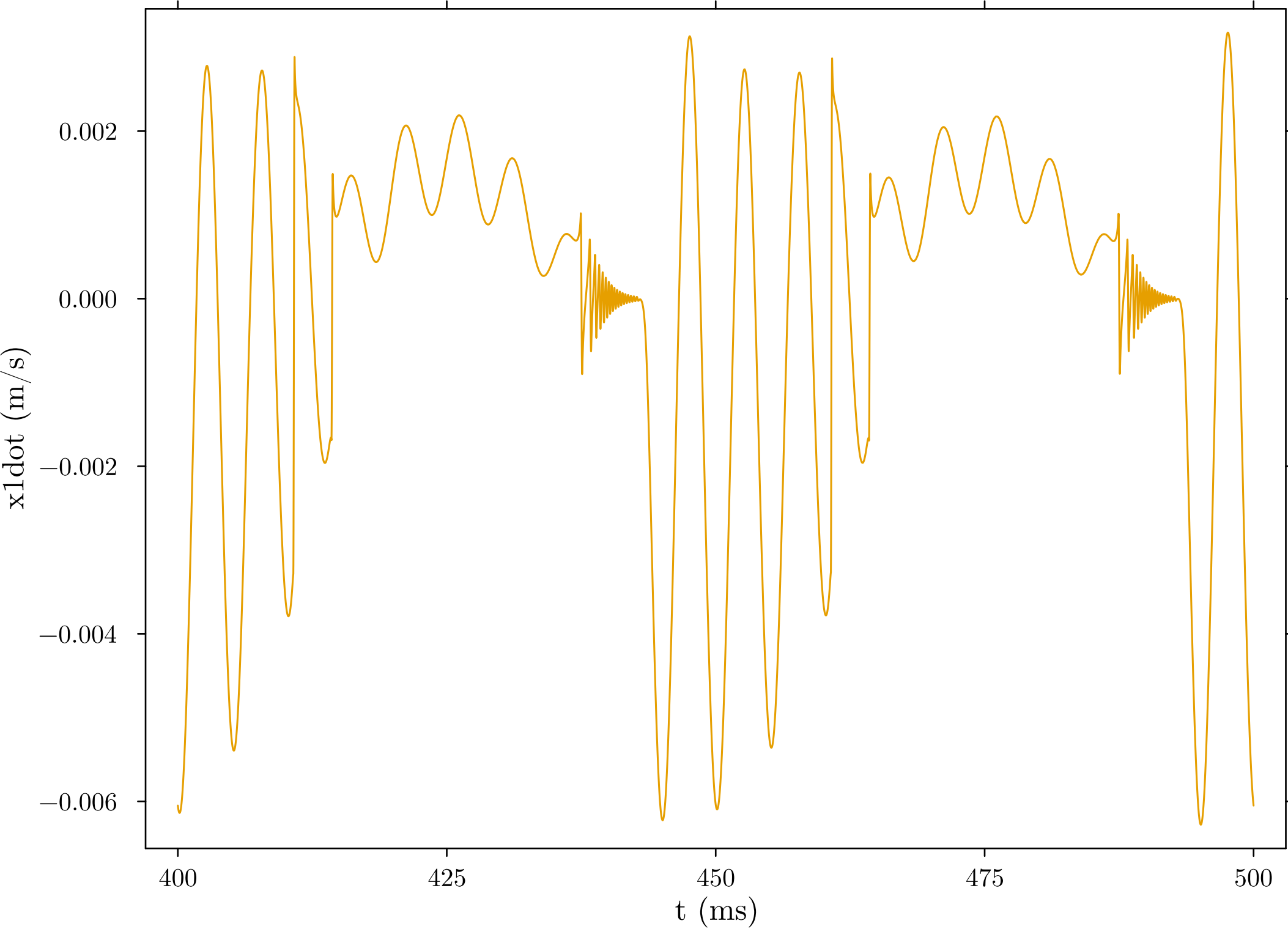
Shuttle Mass Velocity (x1dot) - last 2 cycles
