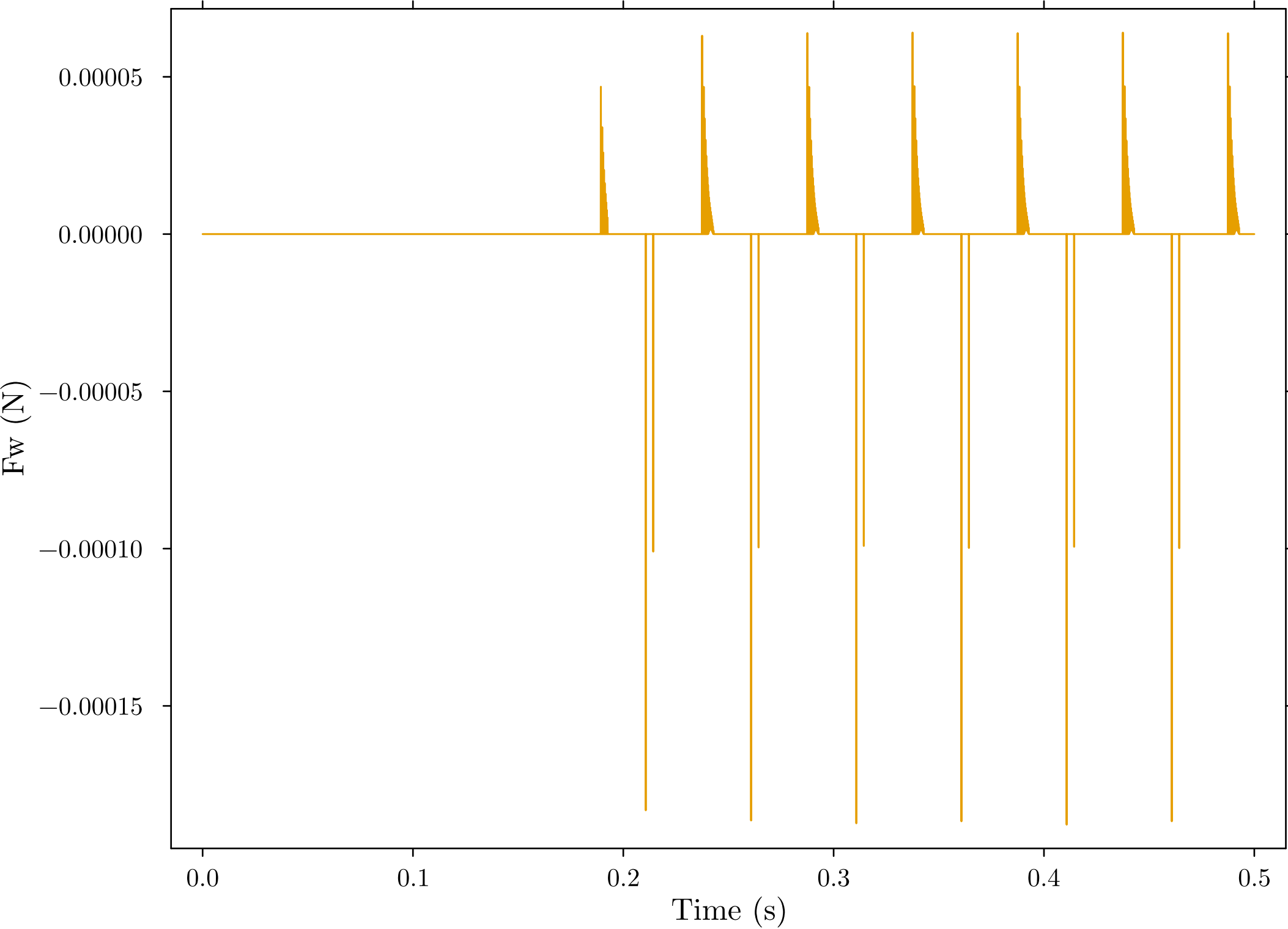
Tip Contact Force on the Tips (reaction on x1 when orient = 1)
