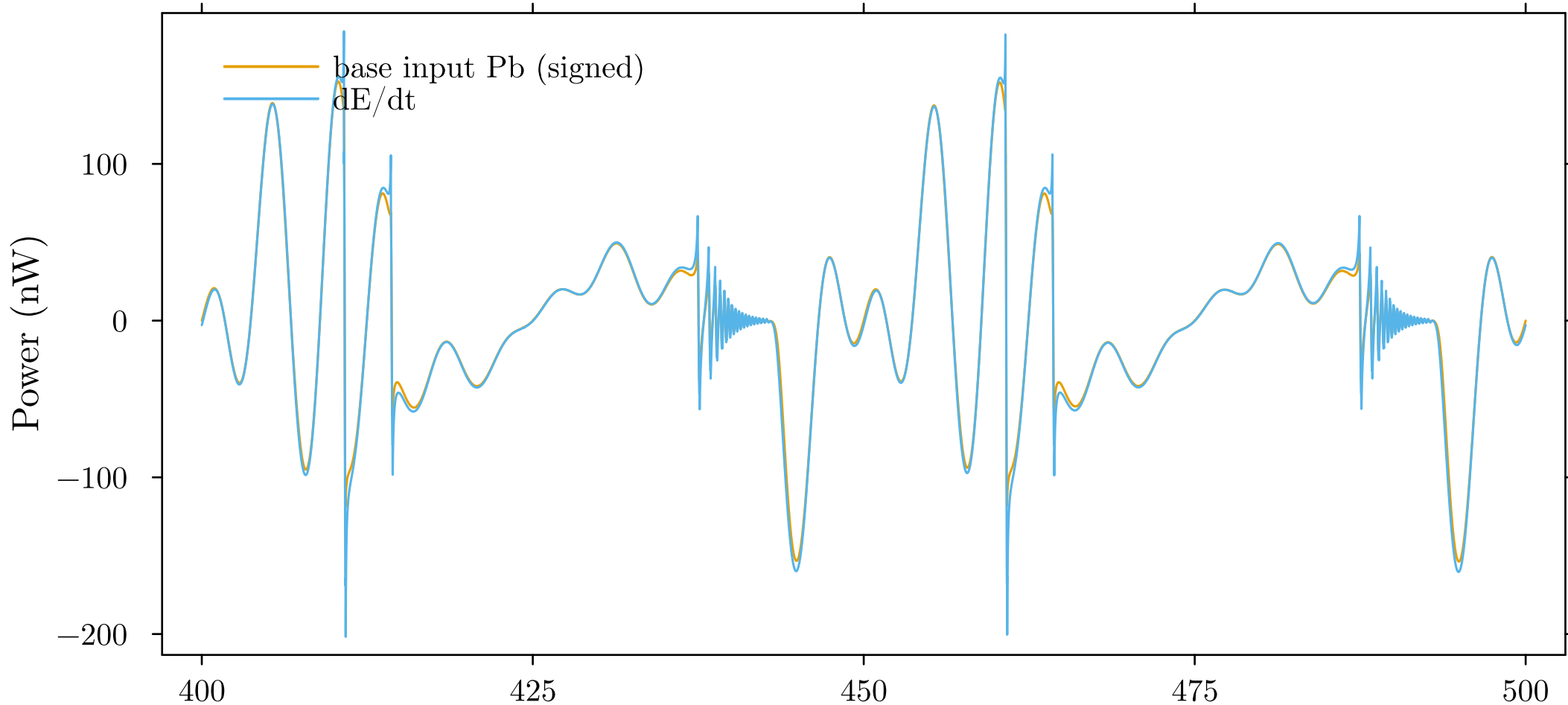
Power Flows - last 2 cycles
