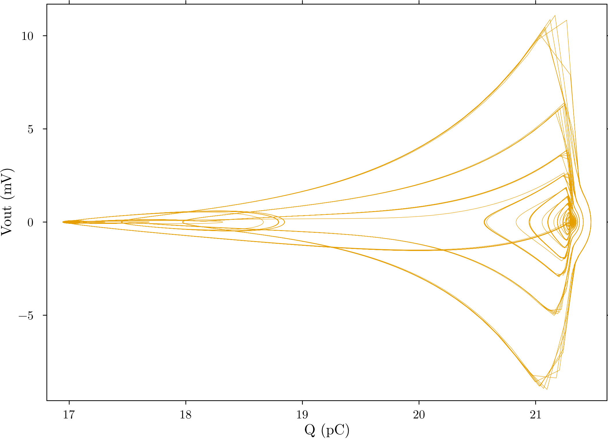
Electrical Plane ( Q , V_{out} ) - full trajectory
