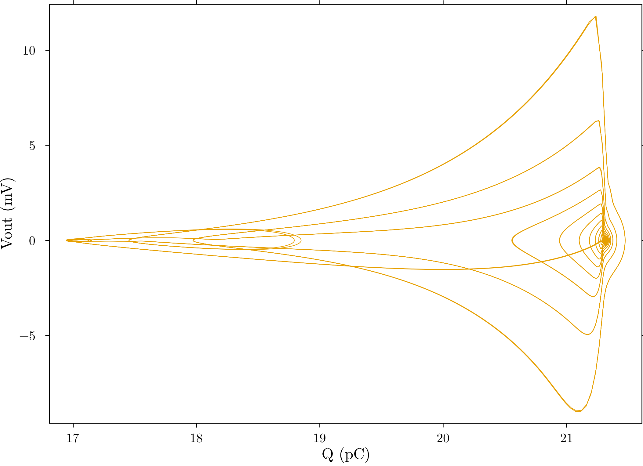
Electrical Plane ( Q , V_{out} ) - last 2 cycles
