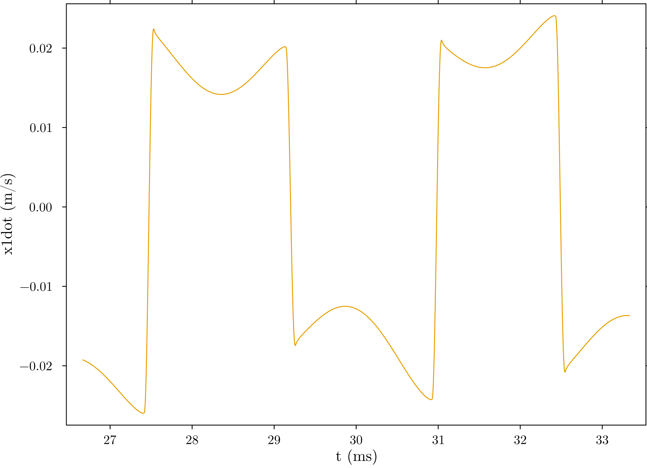
Shuttle Mass Velocity ( \dot{x}_1 ) - last 2 cycles
